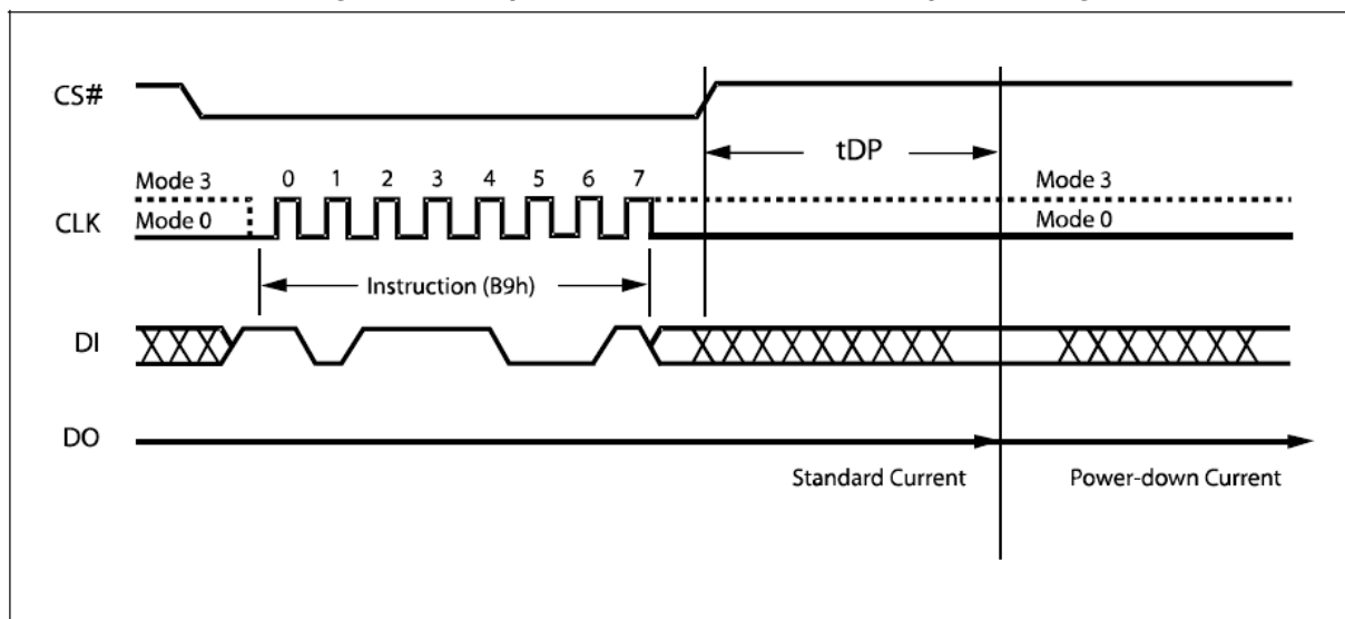
Figure 91. Deep Power-down Instruction Sequence Diagram
