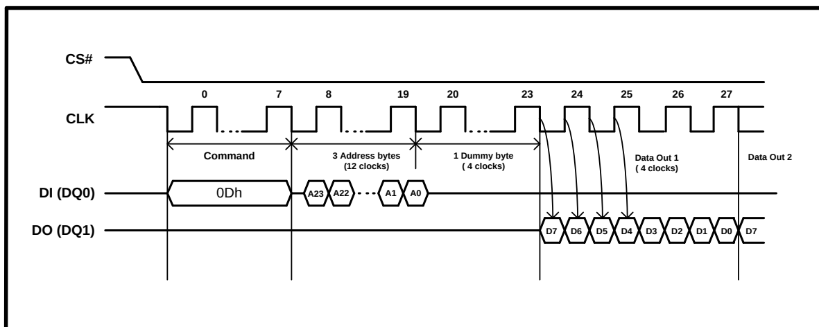
Figure 51. DDR Fast Read Instruction Sequence Diagram
