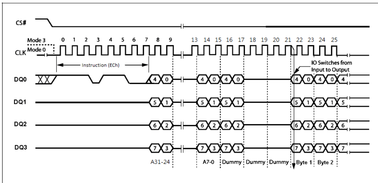
Figure 43. Quad Input / Output Fast Read with 4byte address Instruction Sequence Diagram
