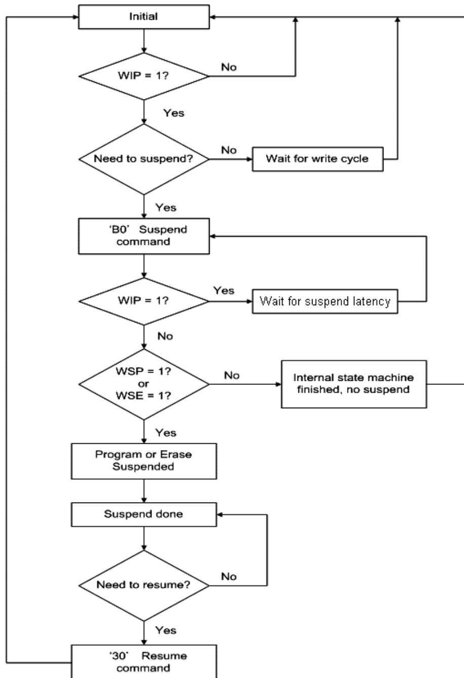
Figure 72. Write Suspend/Resume Flow
