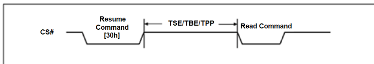
Figure 68. Resume to Read Latency
