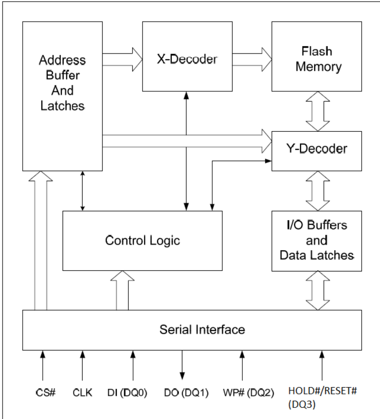
Figure 1. BLOCK DIAGRAM
