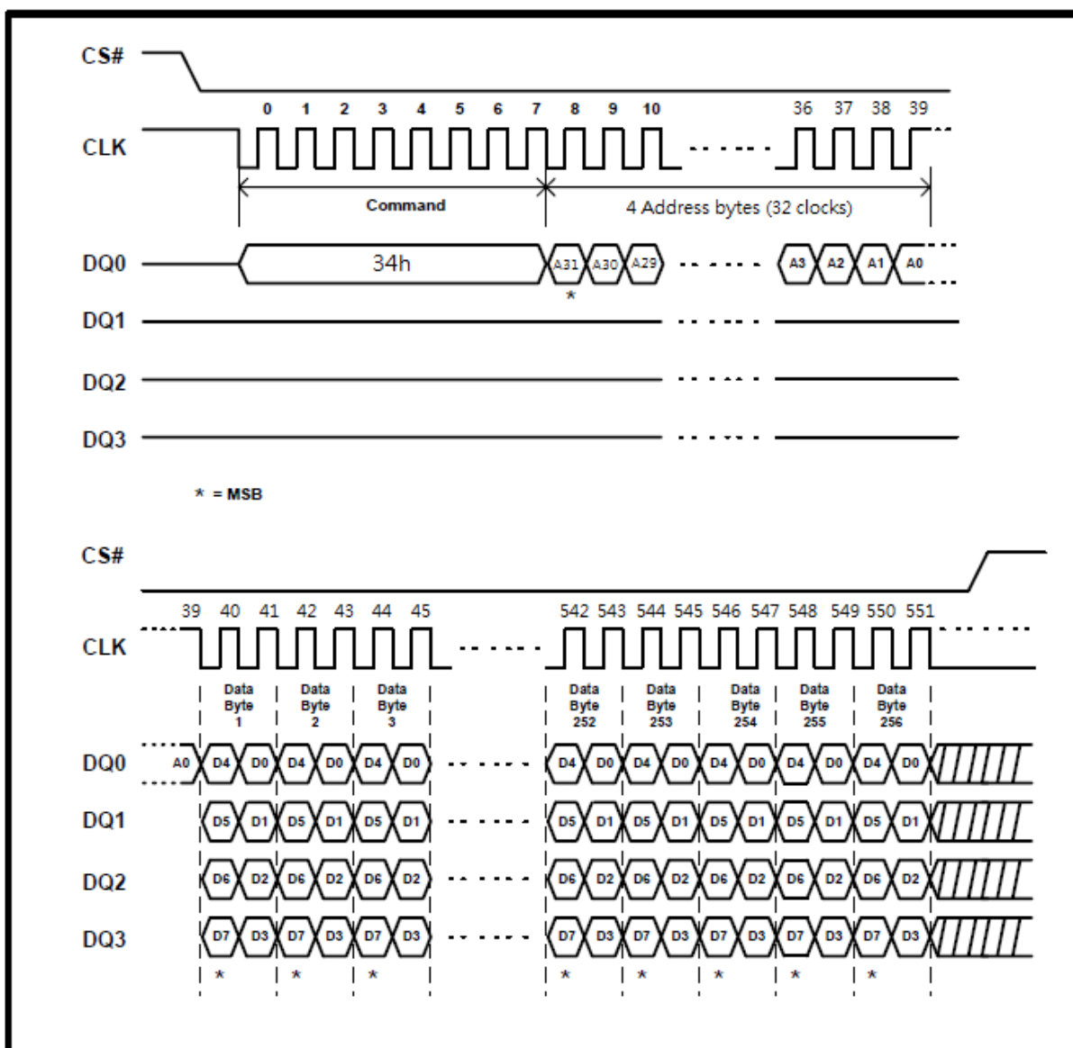
Figure 63. Quad Input Page Program with 4byte address Instruction Sequence Diagram (SPI Mode only)
