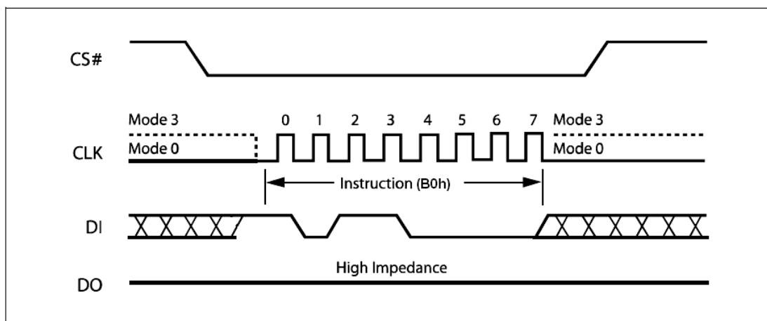
Figure 66. Write Suspend Instruction Sequence Diagram
