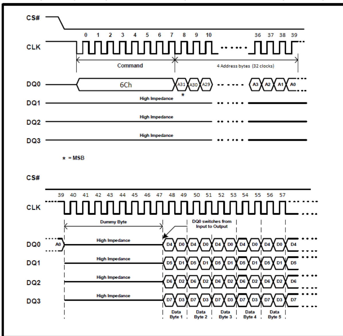
Figure 38. Quad Output Fast Read with 4byte address Instruction Sequence Diagram
