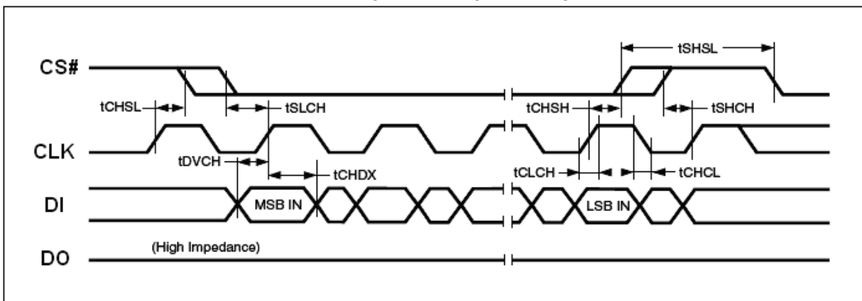
Figure 110. Input Timing
