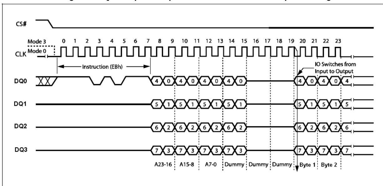
Figure 39. Quad Input / Output Fast Read Instruction Sequence Diagram
