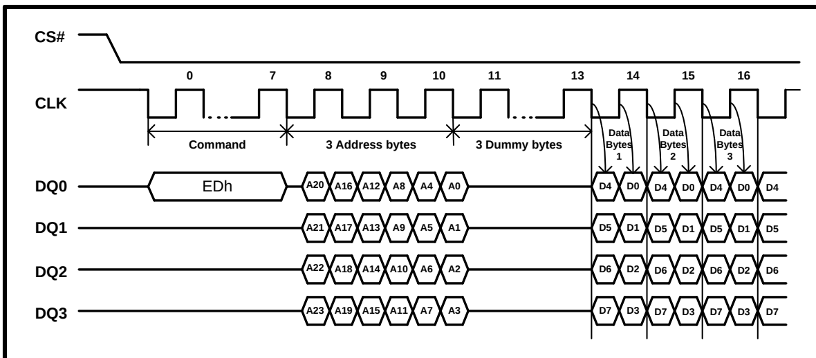
Figure 54. DDR Quad Input / Output FAST_READ Instruction Sequence Diagram
