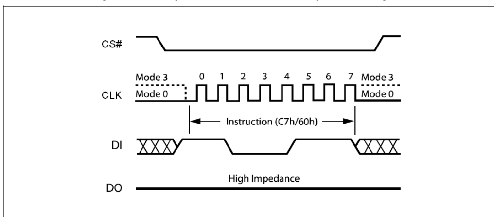
Figure 81. Chip Erase Instruction Sequence Diagram
