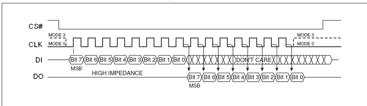
Figure 2. SPI Modes
