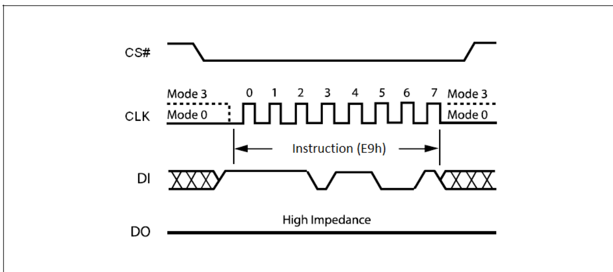
Figure 85. Exit 4byte address mode Instruction Sequence Diagram
