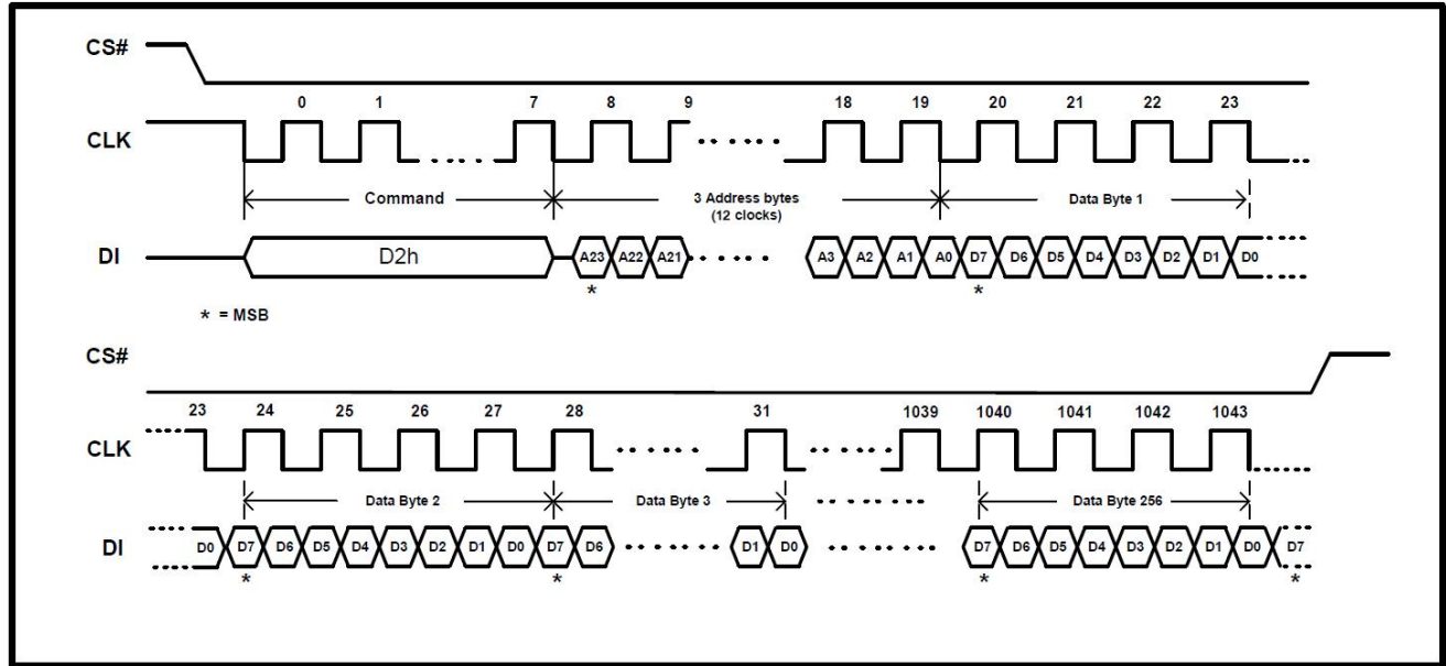
Figure 64. DDR Page Program Instruction Sequence Diagram
