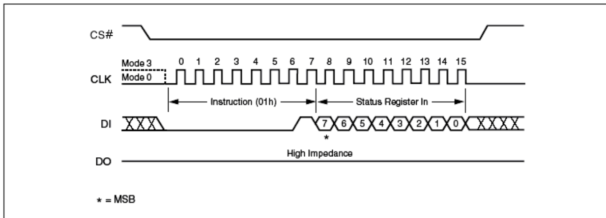
Figure 19. Write Status Register Instruction Sequence Diagram
