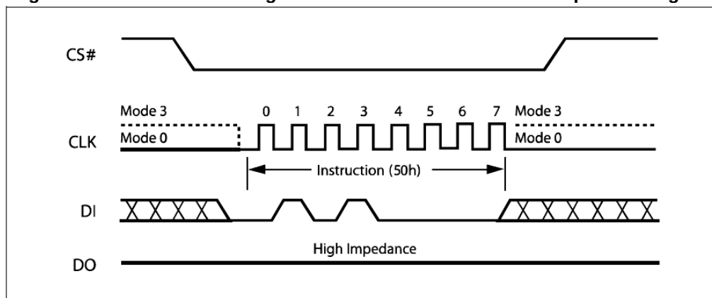
Figure 10. Volatile Status Register Write Enable Instruction Sequence Diagram
