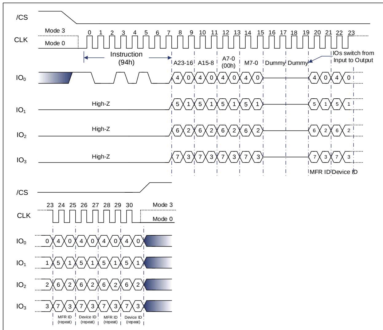
Figure 9-95 Read Manufacturer / Device ID Quad I/O Instruction (SPI Mode only) 32-Bit Address is required when the device is operating in 4-Byte Address Mode
