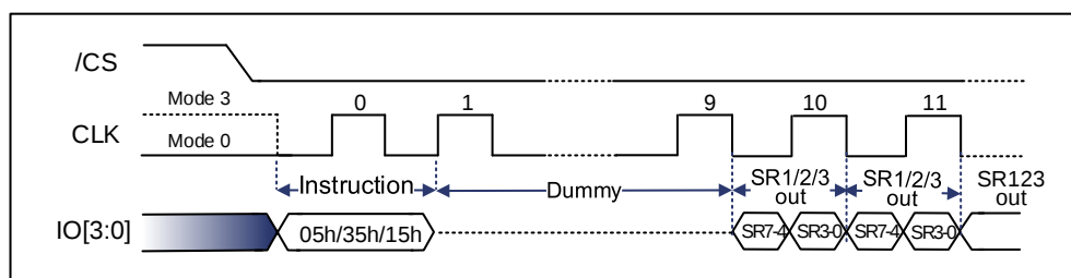
Figure 9-25 Read Status Register Sequence Diagram (Quad DTR)
