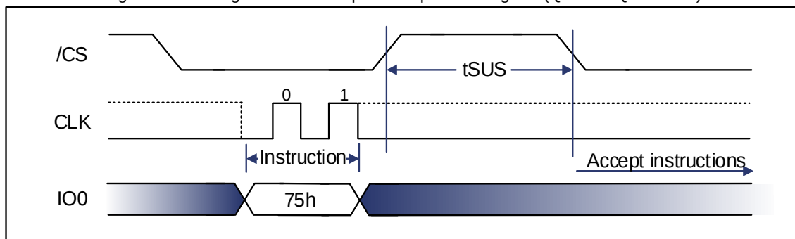
Figure 9-103 Program/Erase Suspend Sequence Diagram (QPI and Quad DTR)
