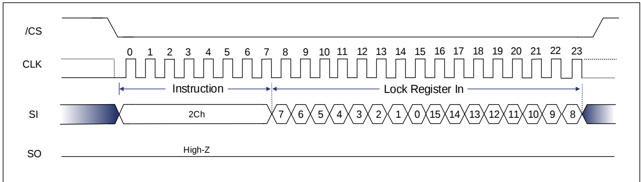
Figure 9-123 Write Lock Register (WRLR) Sequence (SPI Mode)
