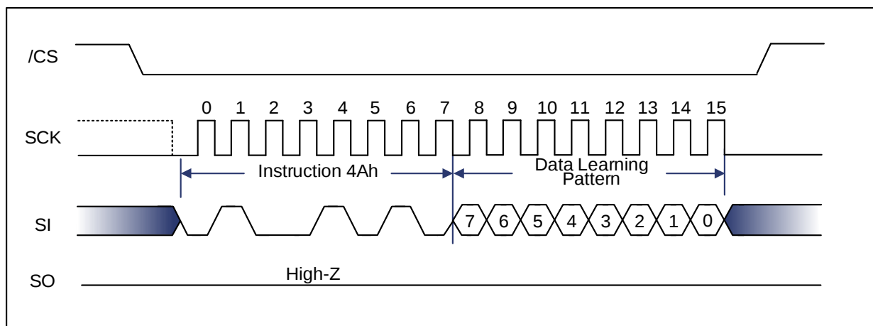
Figure 9-63 Write Data Learning Pattern Sequence Diagram (SPI)
