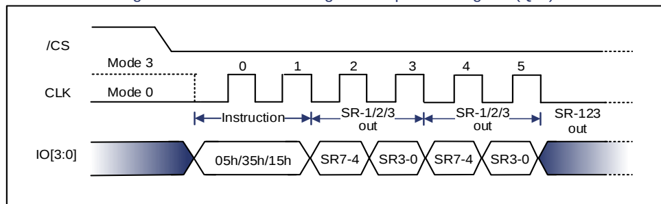
Figure 9-24 Read Status Register Sequence Diagram (QPI)
