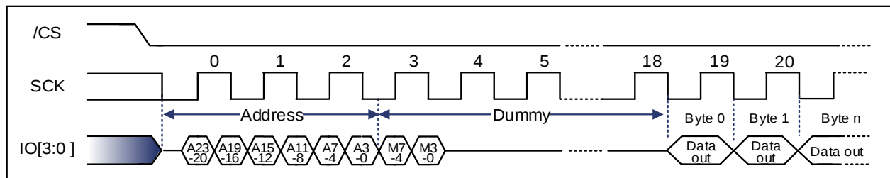
Figure 9-54. DTR Quad I/O Fast Read Sequence Diagram (M5-4 = (1, 0))
