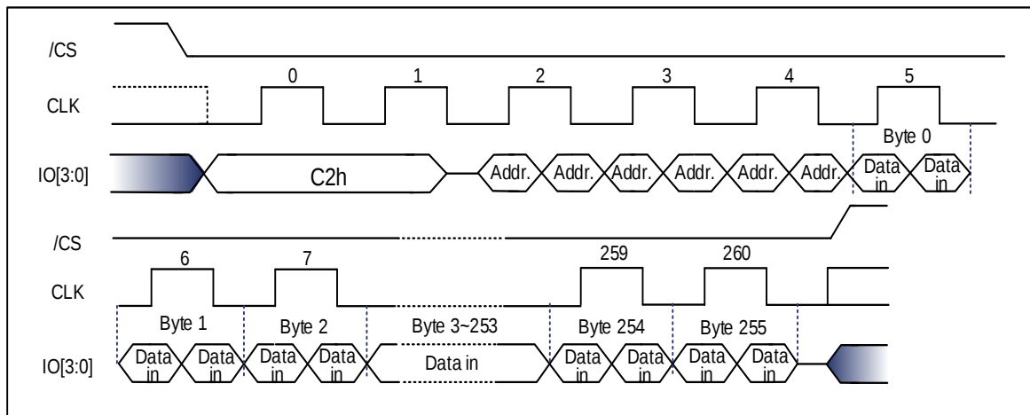
Figure 9-72 Extend Quad Page Program Sequence Diagram (Quad DTR) [1]
