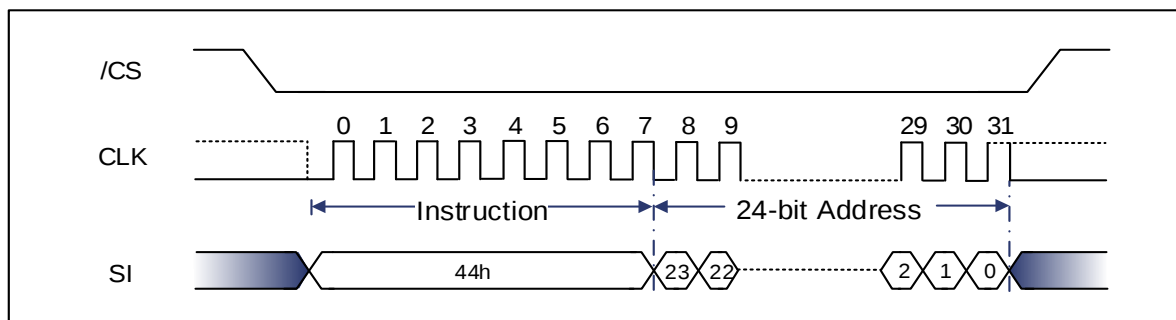
Figure 9-106 Erase Security Registers Command Sequence Diagram (SPI) [1]
