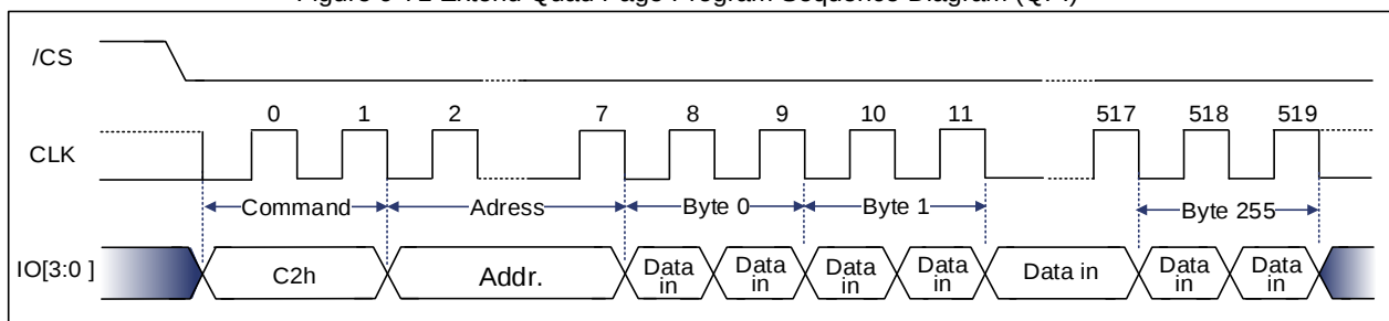
Figure 9-71 Extend Quad Page Program Sequence Diagram (QPI) [1]
