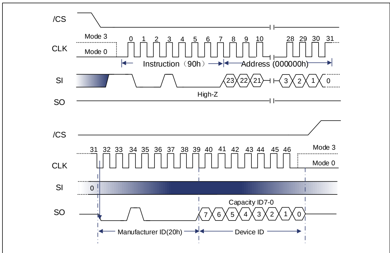
Figure 9-93 Read Manufacturer / Device ID Instruction (SPI Mode)
