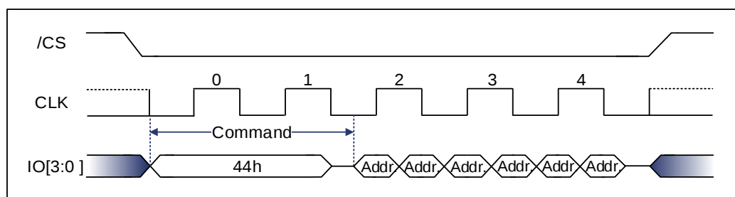
Figure 9-108 Erase Security Registers Command Sequence Diagram (Quad DTR) [1]
