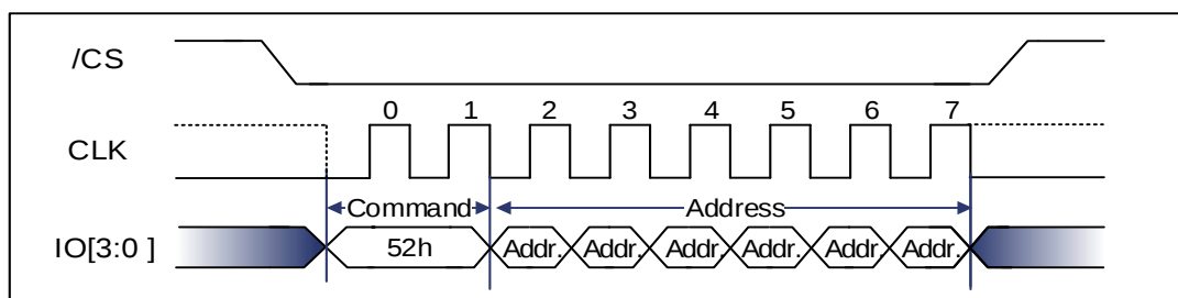
Figure 9-77 32KB Block Erase Sequence Diagram (Quad DTR) [1]
