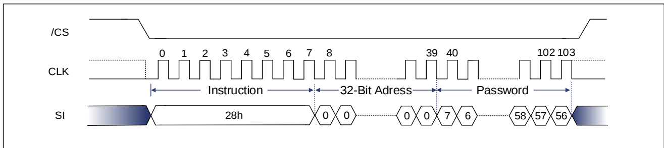
Figure 9-131 Password Unlock (PASSULK) Sequence
