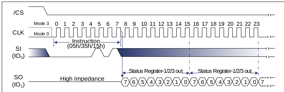
Figure 9-23 Read Status Register Sequence Diagram (SPI)
