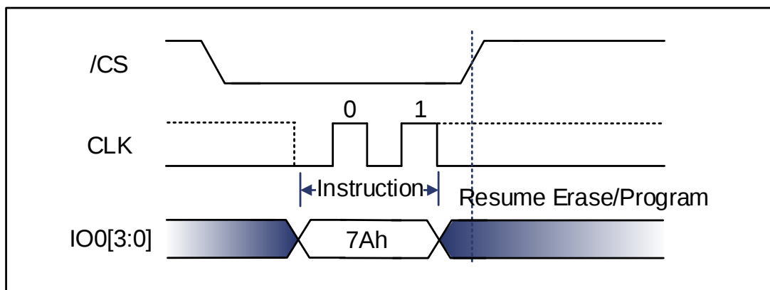
Figure 9-105 Program/Erase Resume Sequence Diagram (QPI and Quad DTR)
