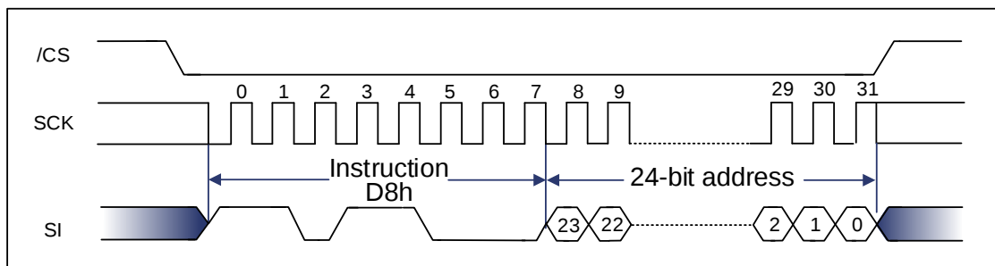
Figure 9-78 64KB Block Erase Sequence Diagram (SPI) [1]
