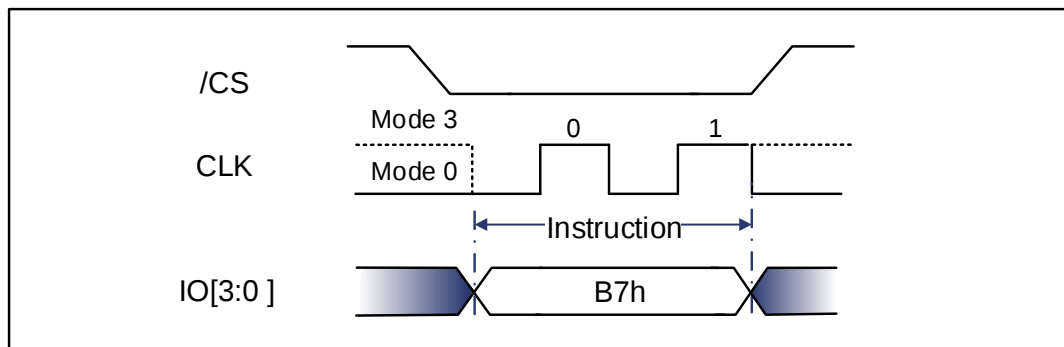
Figure 9-2 Enable 4-Byte Mode Sequence Diagram (QPI and Quad DTR)
