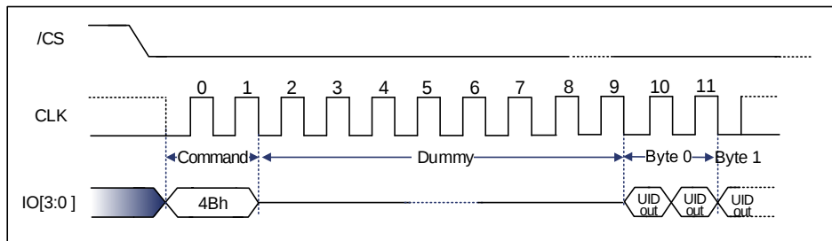
Figure 9-97 Read Unique ID Sequence Diagram (QPI) [1]
