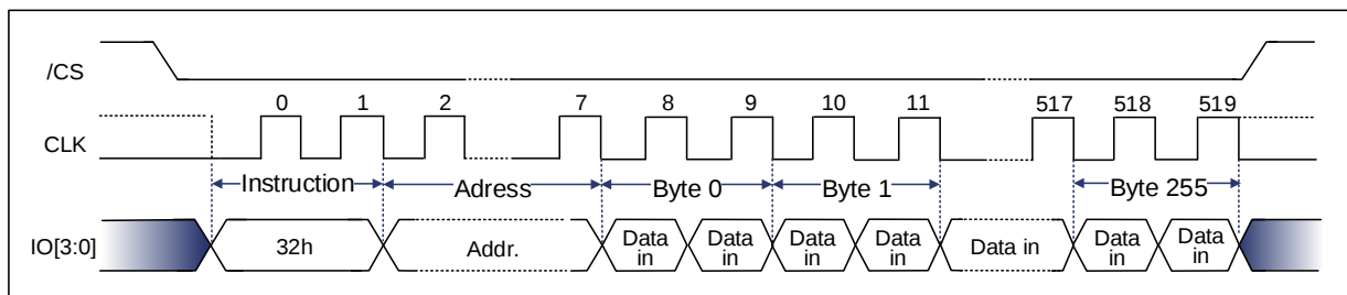
Figure 9-68 Quad Page Program Sequence Diagram (QPI) [1]
