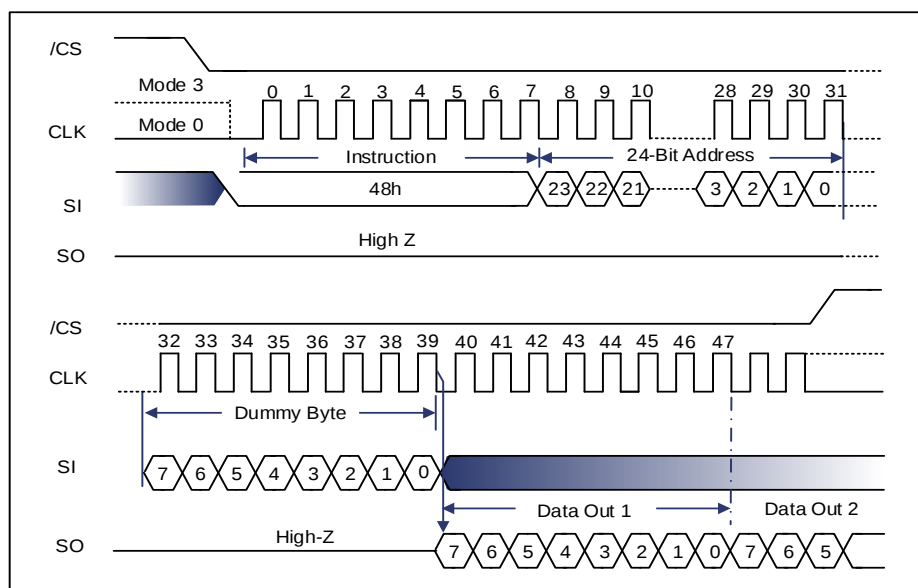
Figure 9-112 Read Security Registers Command Sequence Diagram (SPI) [1]
