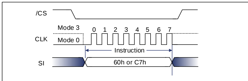
Figure 9-81 Chip Erase Sequence Diagram (SPI)
