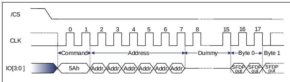
Figure 9-119 Read Serial Flash Discoverable Parameter Command Sequence Diagram (Quad DTR)
