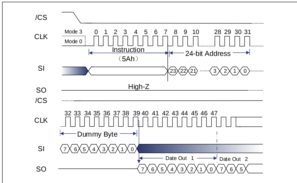
Figure 9-118 Read Serial Flash Discoverable Parameter Command Sequence Diagram (QPI)
