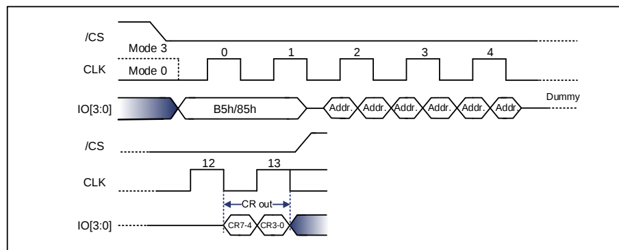
Figure 9-28 Read Configuration Registers Sequence (Quad DTR) [1]
