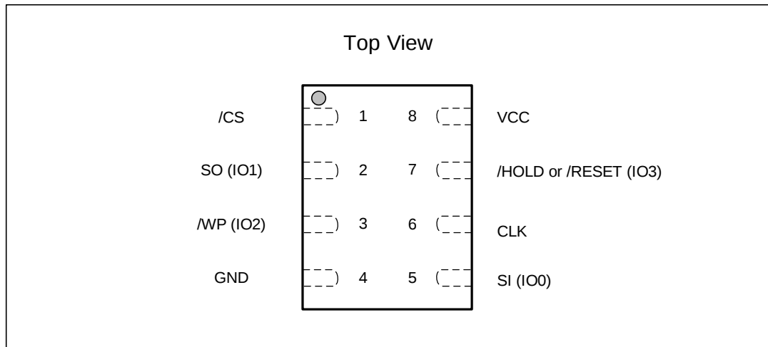
Figure 2-2 8-pin WSON (Package Code X)
