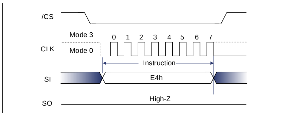
Figure 9-125 SPB Erase (ESSPB) Sequence
