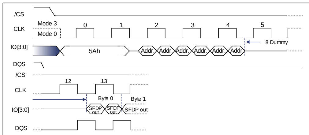
Figure 9-119 Read Serial Flash Discoverable Parameter Command Sequence Diagram (Quad DTR)
