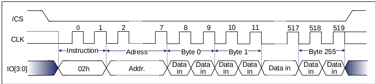
Figure 9-65 Page Program Sequence Diagram (QPI) [1]
