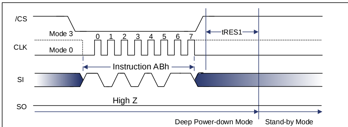
Figure 9-88 Release Power-Down Sequence Diagram (SPI)
