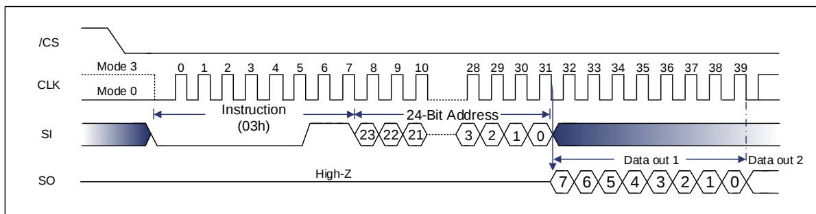
Figure 9-32 Read Data Bytes Sequence Diagram [1]
