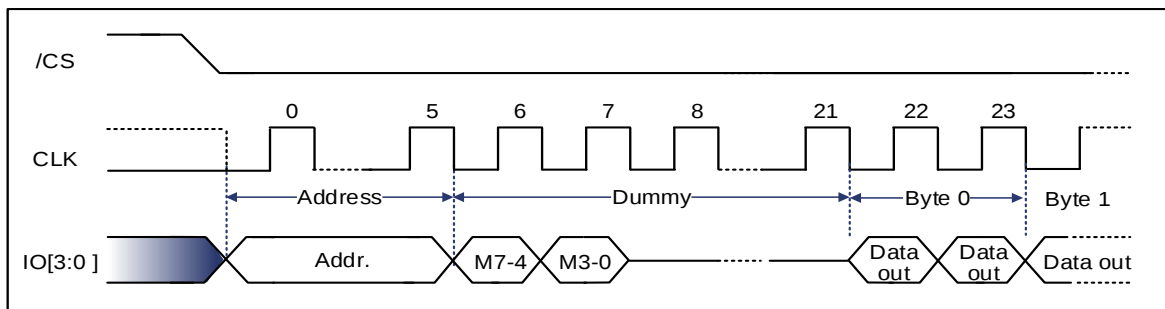
Figure 9-49 Quad I/O Fast Read Sequence Diagram (STR, M5-4= (1, 0)) [1]
