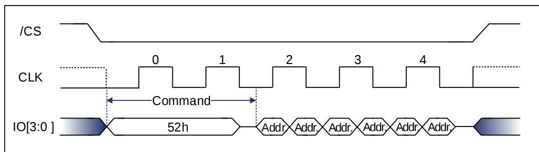
Figure 9-77 32KB Block Erase Sequence Diagram (Quad DTR) [1]
