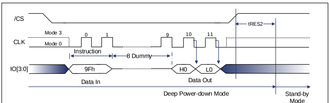
Figure 9-92 Release Power-Down/Read Device ID Sequence Diagram (Quad DTR)
