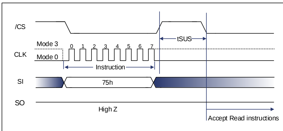
Figure 9-102 Program/Erase Suspend Sequence Diagram (SPI)
