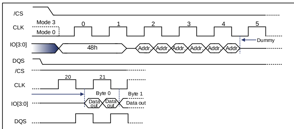
Figure 9-114 Read Security Registers Command Sequence Diagram (Quad DTR) [1]
