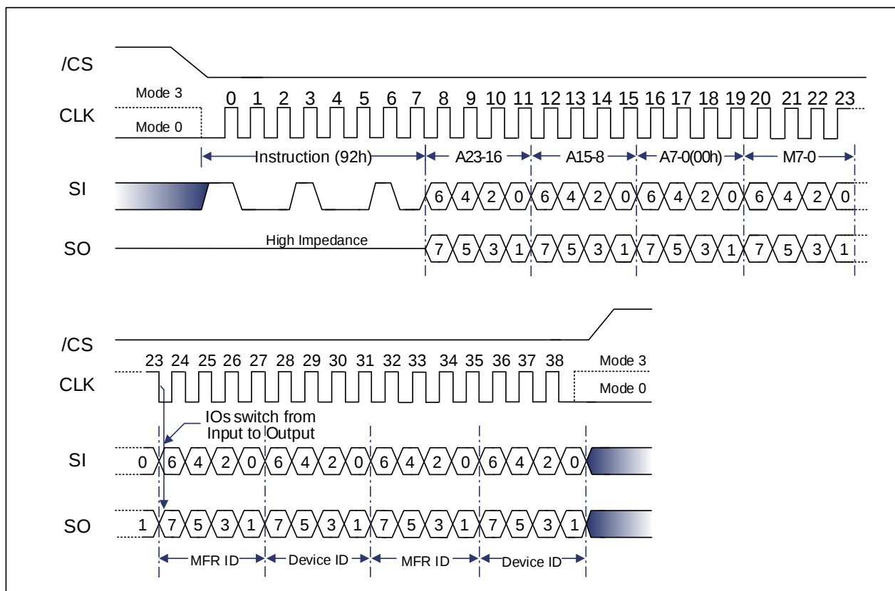
Figure 9-94 Read Manufacturer / Device ID Dual I/O Instruction (SPI Mode only) 32-Bit Address is required when the device is operating in 4-Byte Address Mode
