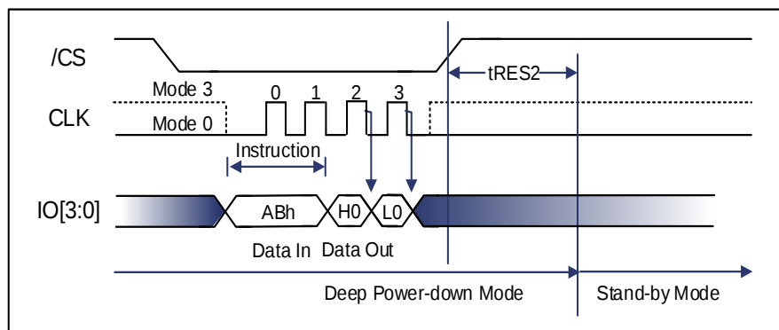
Figure 9-91 Release Power-Down/Read Device ID Sequence Diagram (QPI)
