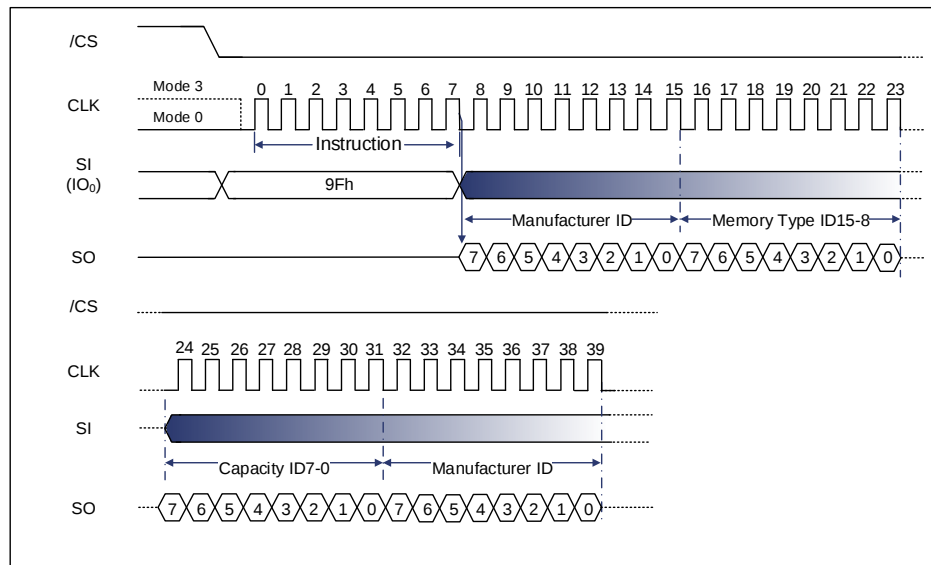
Figure 9-100 Read Identification ID Sequence Diagram (QPI)
