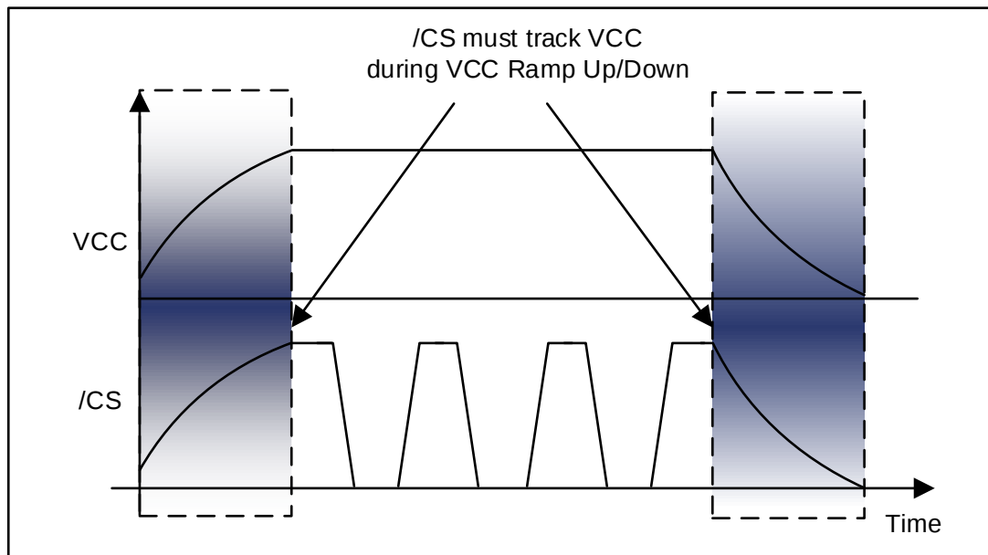
Figure 10-2 Power-up, Power-Down Requirement
