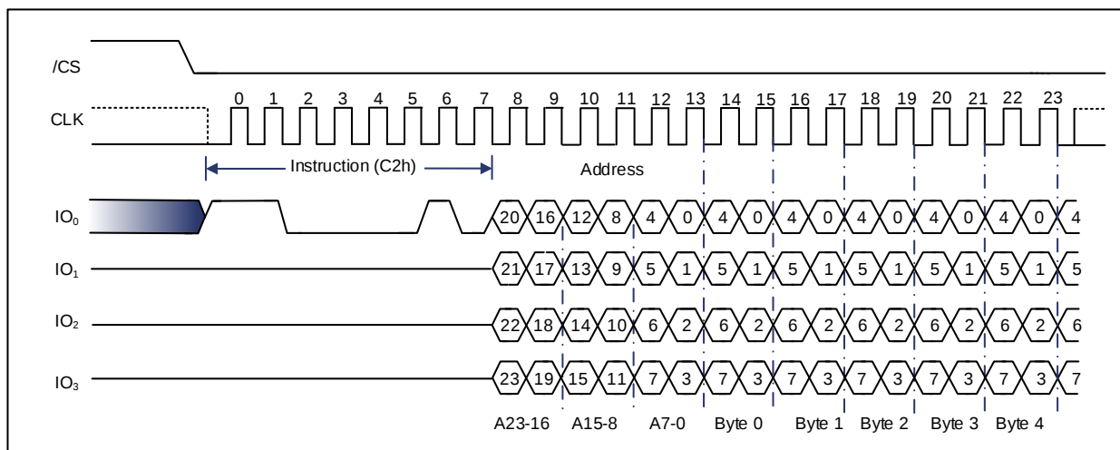
Figure 9-70 Extend Quad Page Program Sequence Diagram (SPI) [1]
