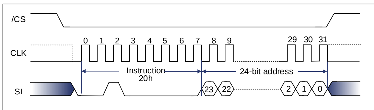
Figure 9-73 Sector Erase Sequence Diagram (SPI) [1]
