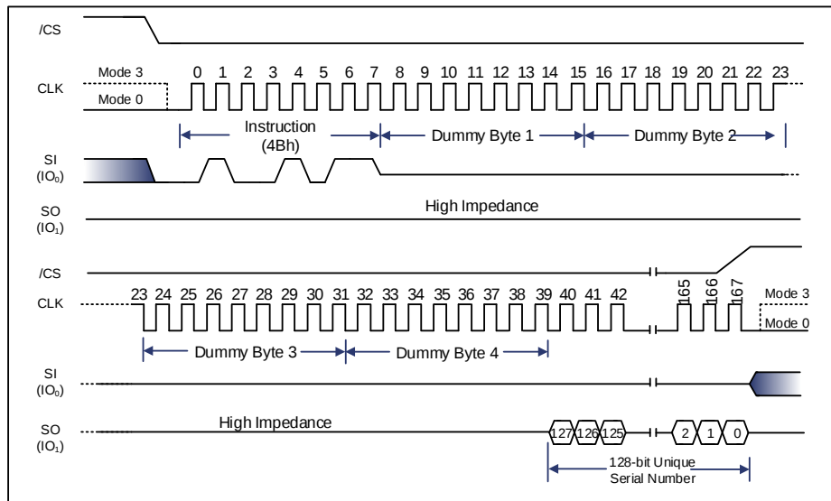
Figure 9-96 Read Unique ID Sequence Diagram (SPI) [1]
