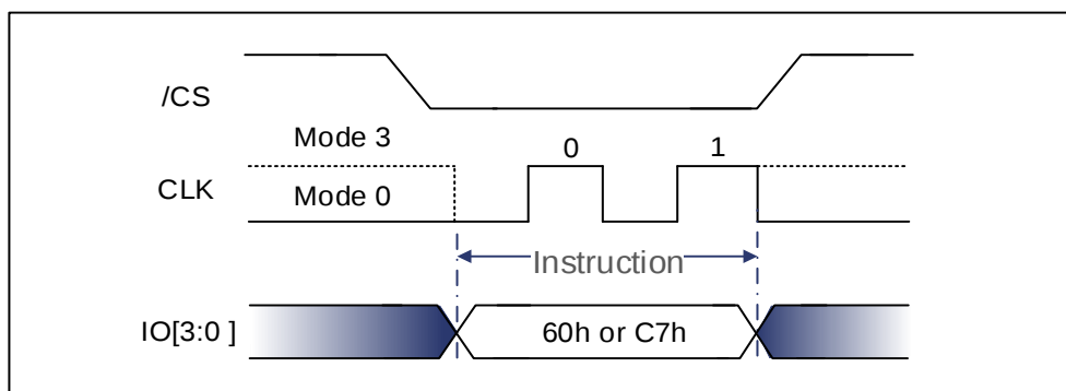
Figure 9-82 Chip Erase Sequence Diagram (QPI and Quad DTR)
