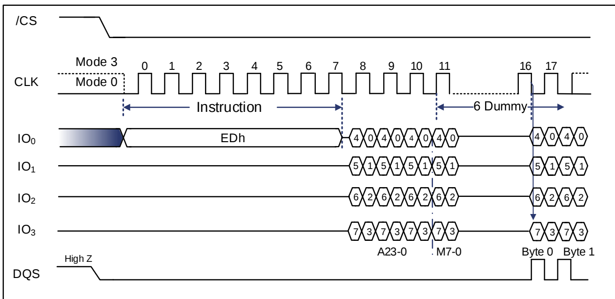
Figure 9-51. DTR Quad I/O Fast Read Sequence Diagram (SPI, M5-4 ≠ (1, 0)) [1]
