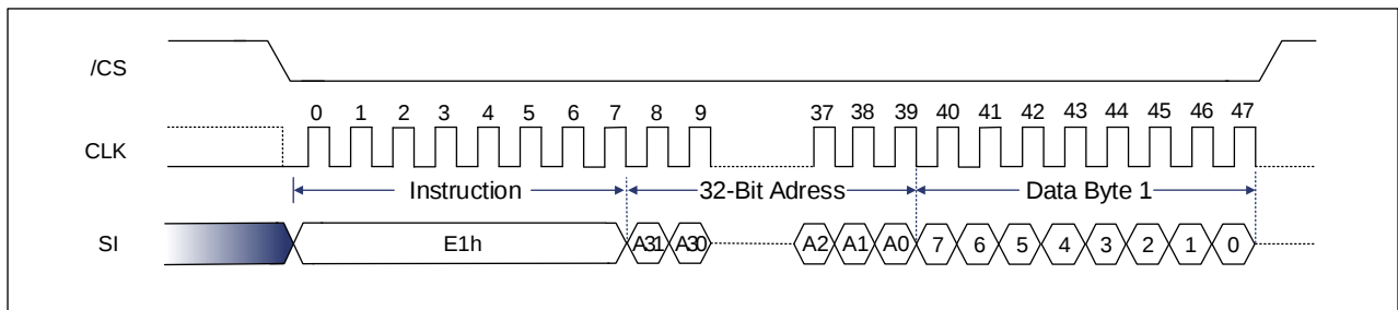
Figure 9-128 Write DPB Register (WRDPB) Sequence
