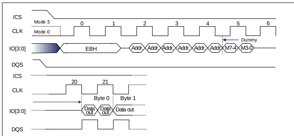
Figure 9-48 Quad I/O Fast Read Sequence Diagram (Quad DTR, M5-4≠ (1, 0)) [1]
