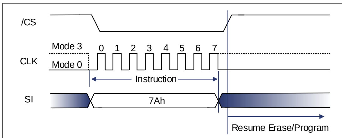
Figure 9-104 Program/Erase Resume Sequence Diagram(SPI)
