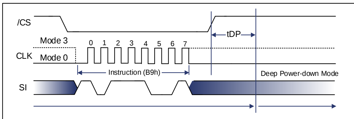
Figure 9-86 Deep Power-Down Sequence Diagram (SPI)
