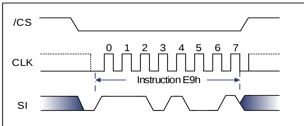
Figure 9-3 Disable 4-Byte Mode Sequence Diagram (SPI)
