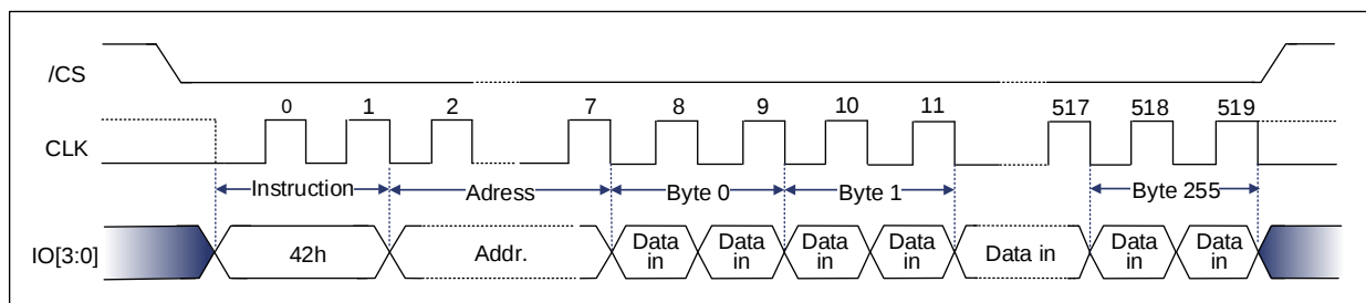
Figure 9-110 Program Security Registers Command Sequence Diagram (QPI) [1]
