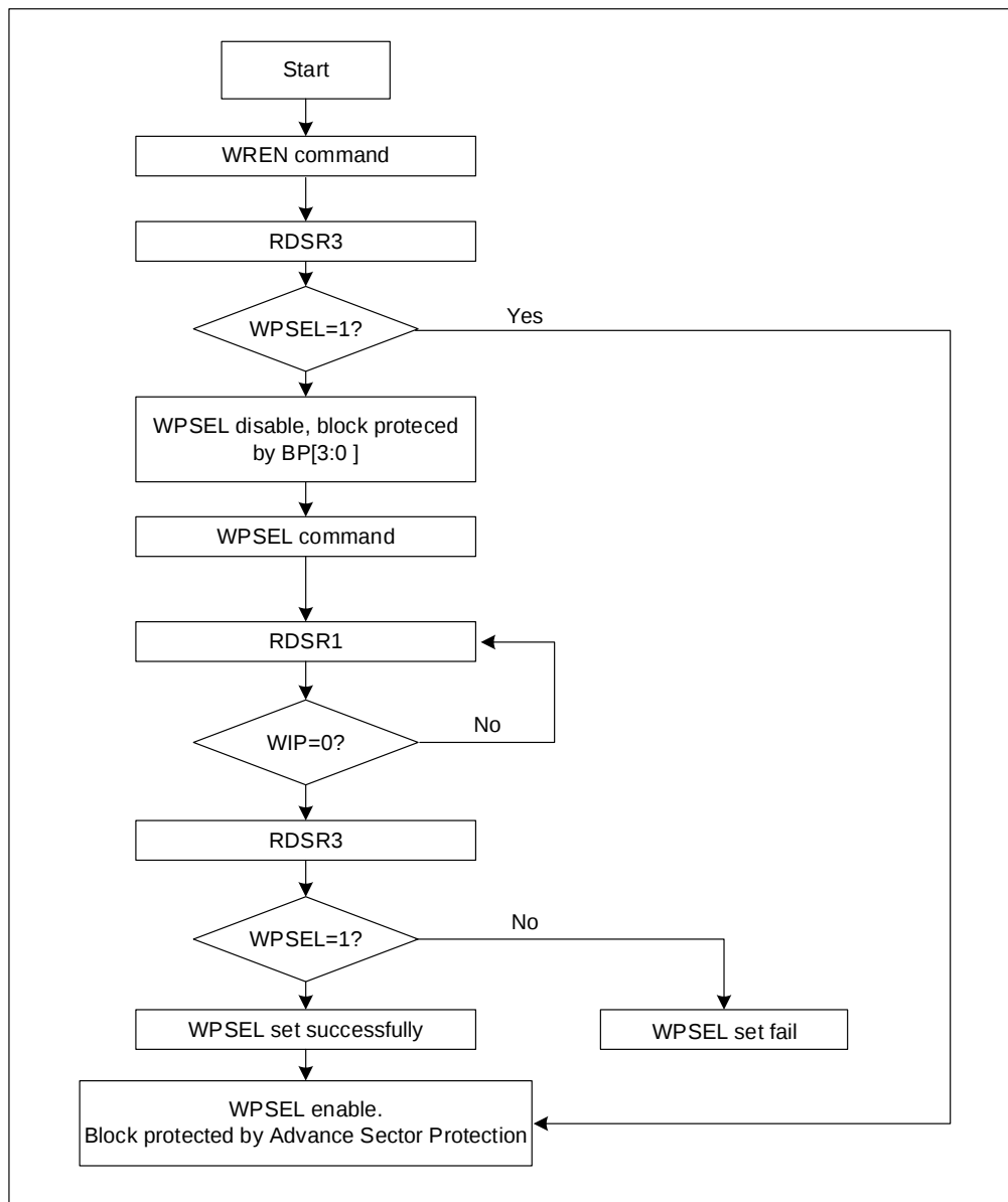
WPSEL Flow
