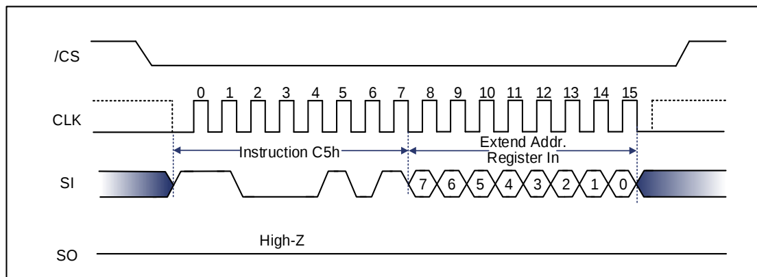
Figure 9-17 Write Extended Address Register Sequence Diagram (SPI)
