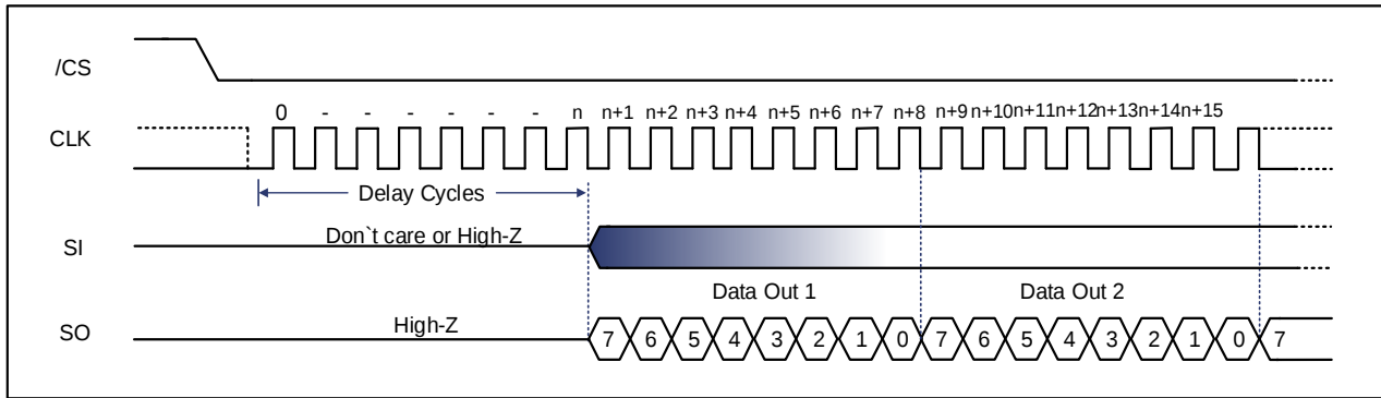
Figure 9-138 Fast Boot Sequence (QE=0)
