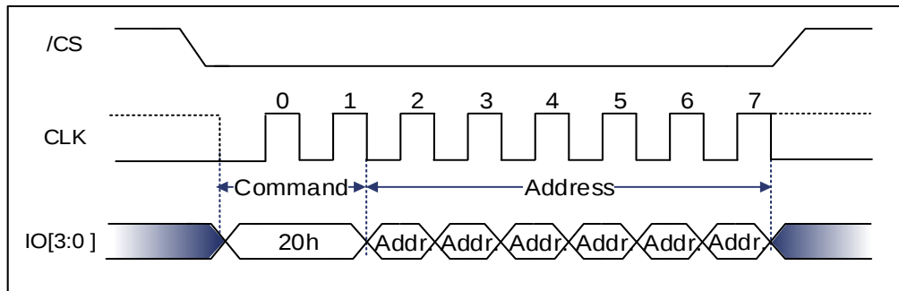
Figure 9-74 Sector Erase Sequence Diagram (QPI) [1]
