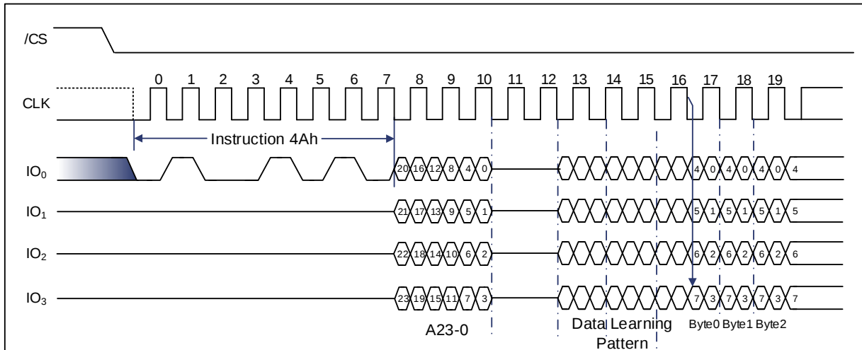
Figure 9-62 Data Learning Pattern Output Sequence Diagram
