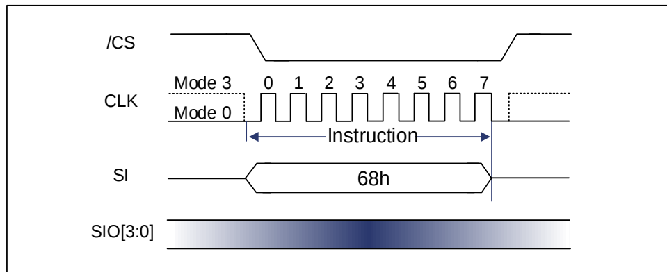
Figure 9-120 WPSEL Command Timing
