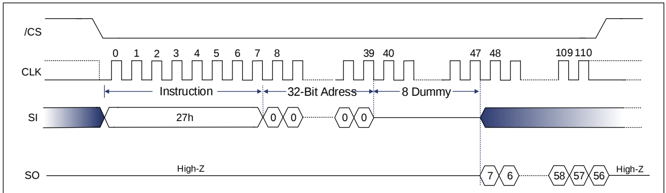
Figure 9-130 Write Password Register (WRPASS) Sequence
