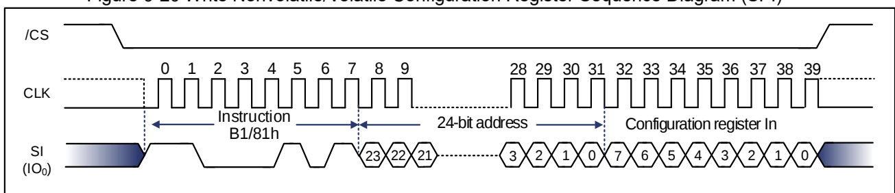
Figure 9-20 Write Nonvolatile/Volatile Configuration Register Sequence Diagram (SPI) [1]
