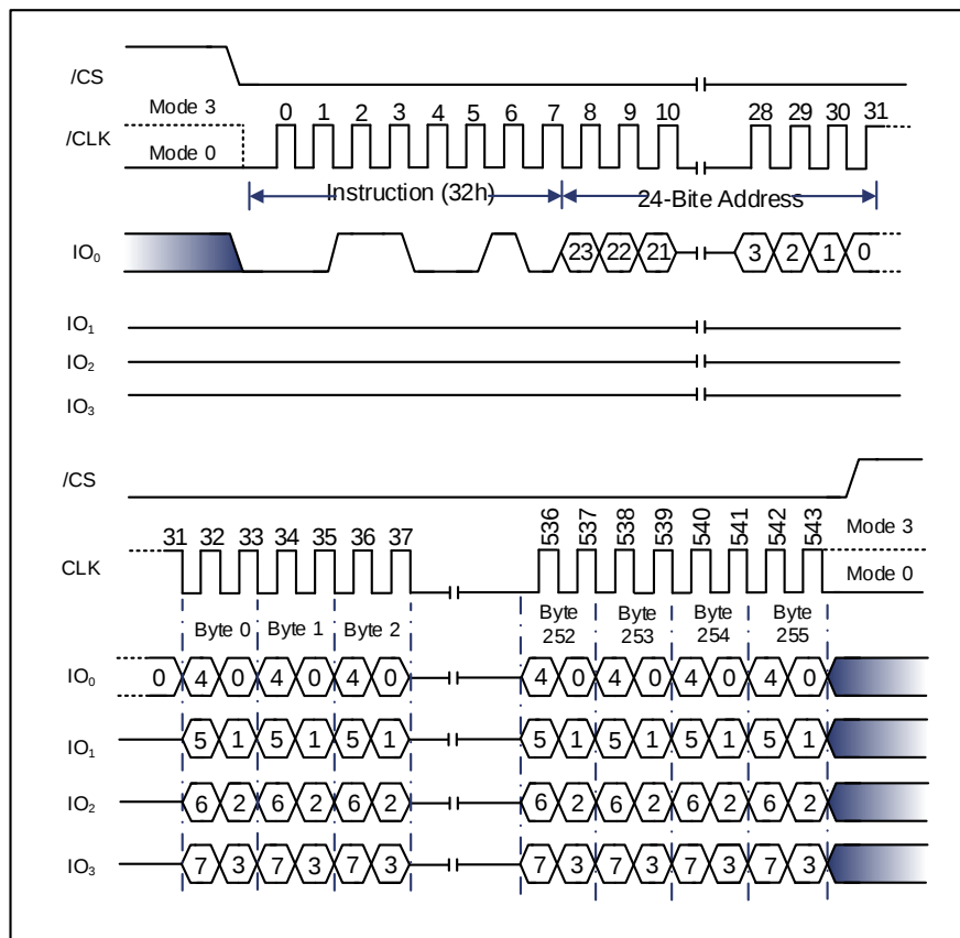
Figure 9-67 Quad Page Program Sequence Diagram (SPI) [1]
