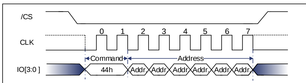
Figure 9-107 Erase Security Registers Command Sequence Diagram (QPI) [1]
