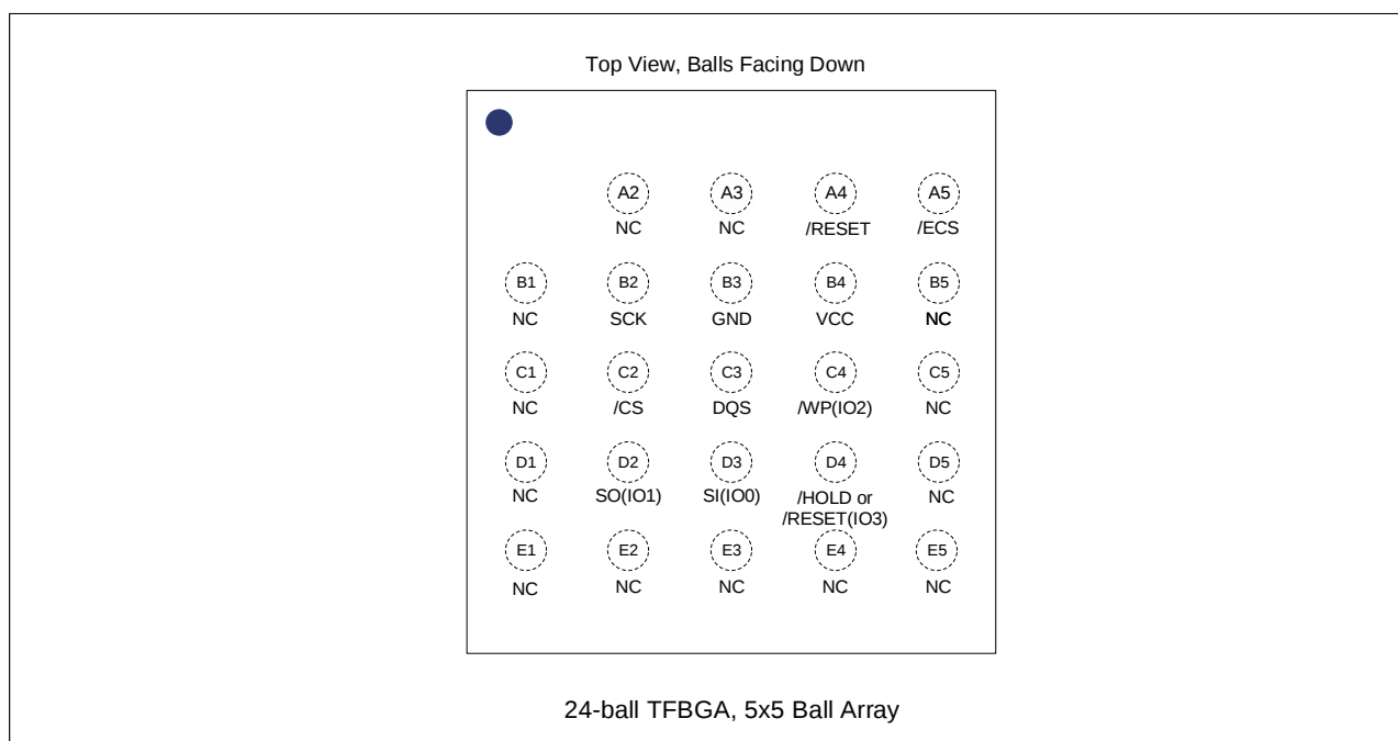
Figure 2-3 TFBGA 8x6-mm 24-ball (Package Code B2, 5x5 ball array)
