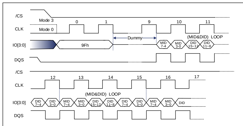
Figure 9-101 Read Identification ID Sequence Diagram (Quad DTR)
