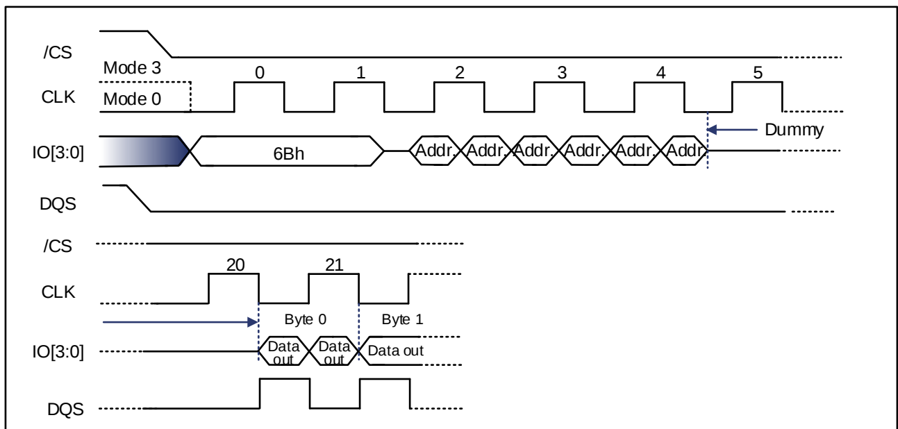
Figure 9-41 Quad Output Fast Read Sequence Diagram (Quad DTR) [1]
