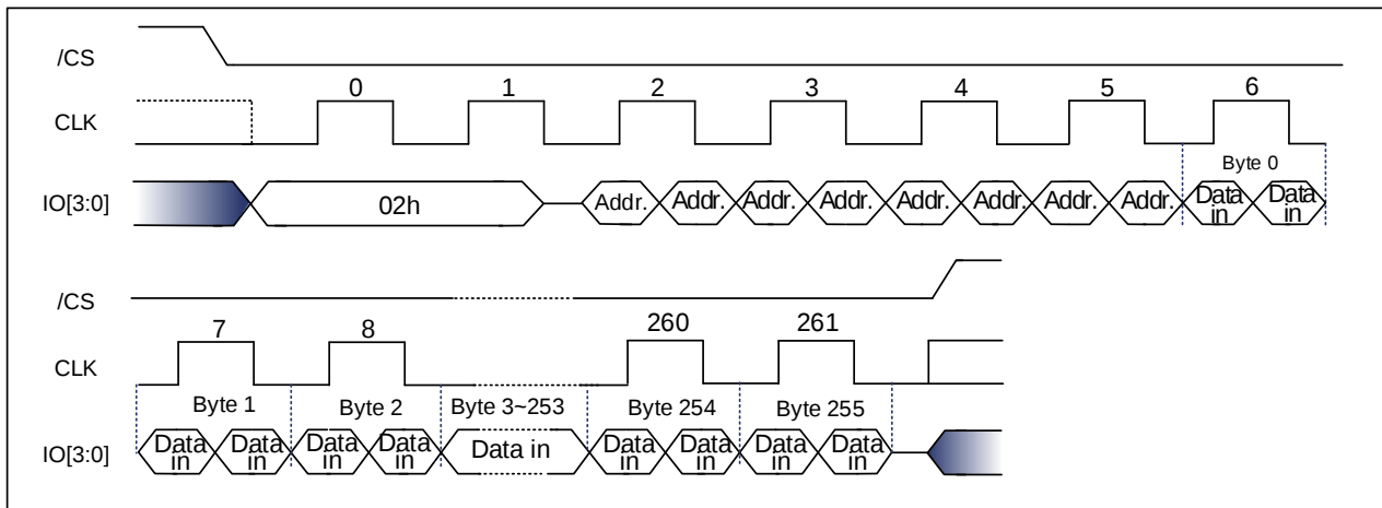
Figure 9-66 Page Program Sequence Diagram (Quad DTR) [1]
