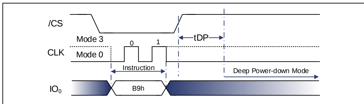
Figure 9-87 Deep Power-Down Sequence Diagram (QPI and Quad DTR)
