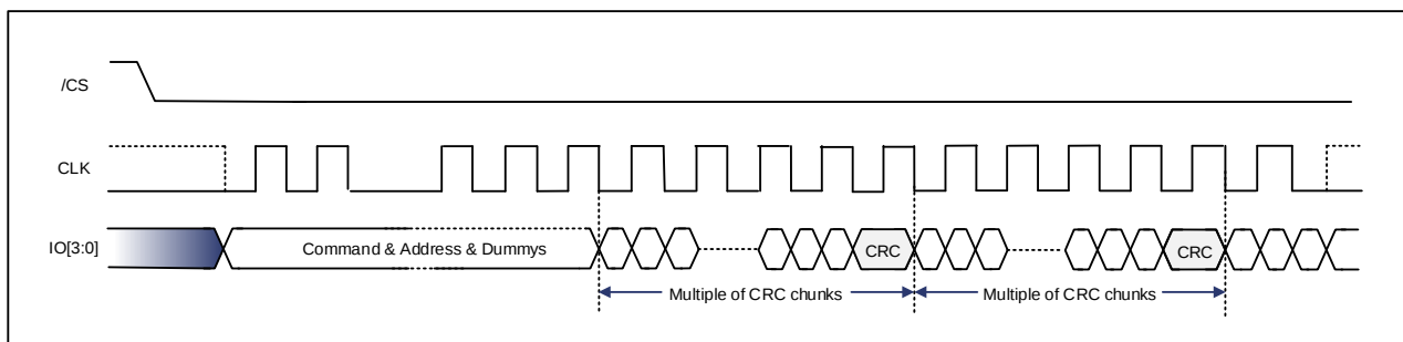
Figure 7-1 CRC Timing
