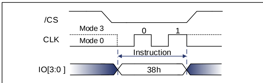
Figure 9-84 Enable QPI mode command Sequence Diagram (Quad DTR)
