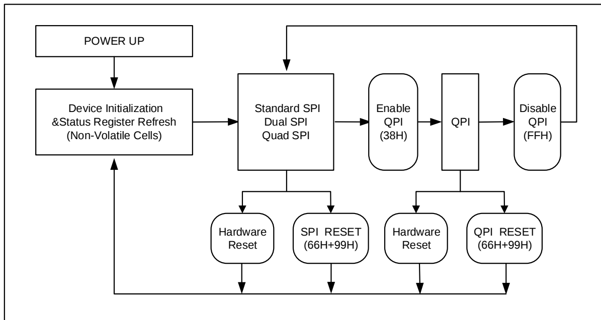
Figure 4-1 XM25EU256D Serial Flash Memory Operation Diagram
