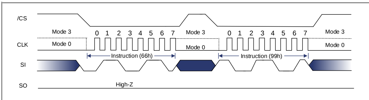
Figure 9-115 Enable Reset and Reset Command Sequence Diagram (SPI)
