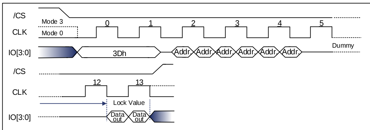
Figure 9-137 Read Individual Block/Sector lock command Sequence Diagram (Quad DTR)
