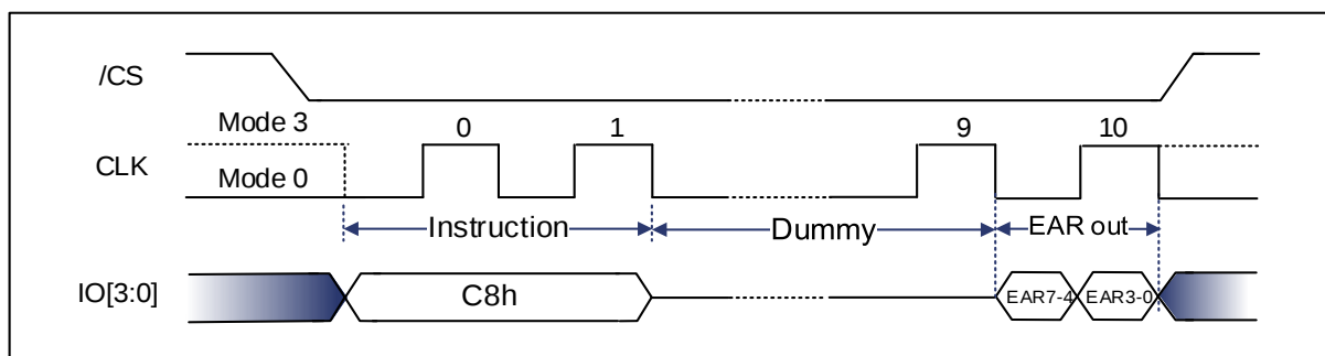
Figure 9-31 Read Extended Address Register Sequence Diagram (Quad DTR) [1]
