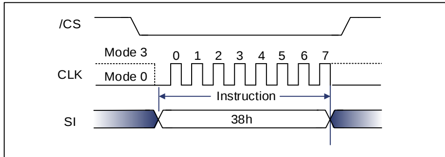
Figure 9-83 Enable QPI mode command Sequence Diagram (SPI)
