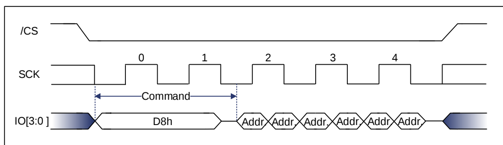
Figure 9-80 64KB Block Erase Sequence Diagram (Quad DTR) [1]
