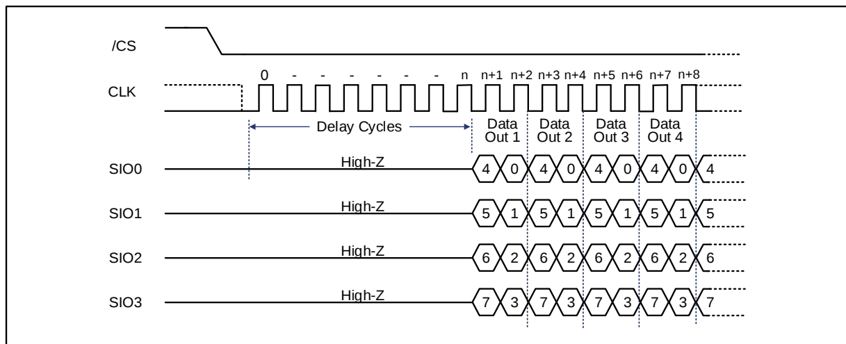
Figure 9-139 Fast Boot Sequence (QE=1)
