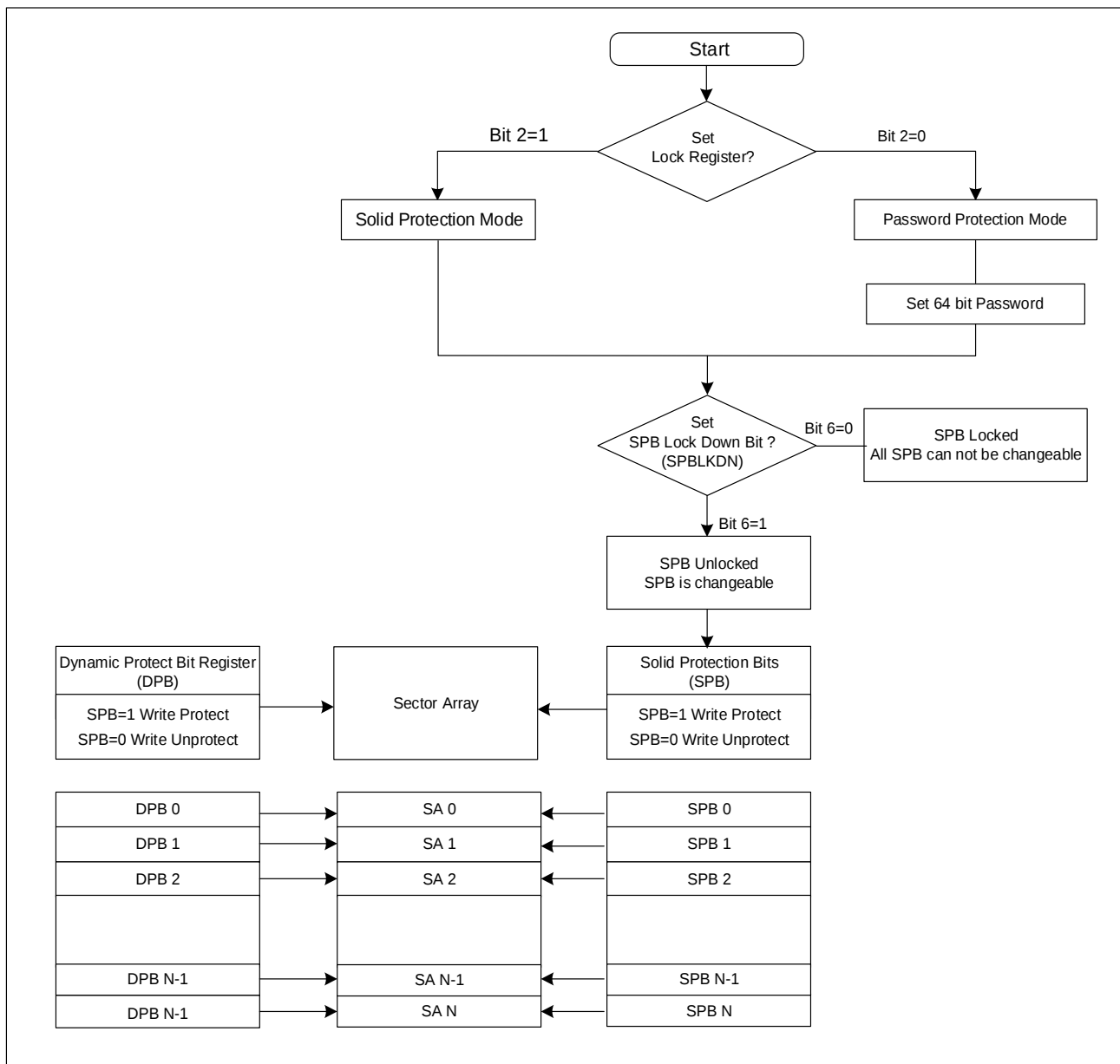
Figure 9-121 The detail algorithm of advanced sector protection
