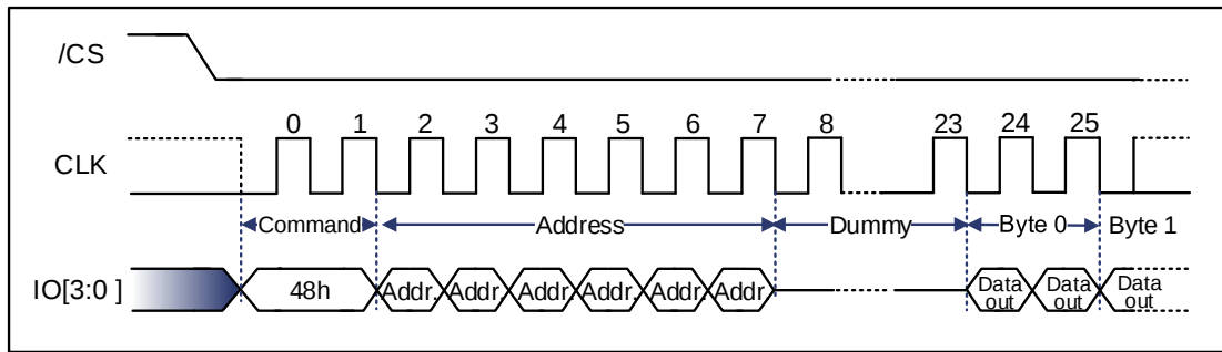
Figure 9-113 Read Security Registers Command Sequence Diagram (QPI) [1]
