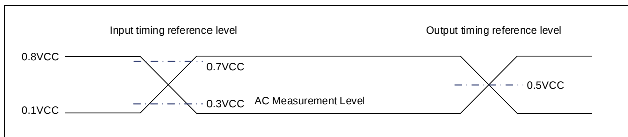
Figure 10-5. Absolute Maximum Ratings Diagram
