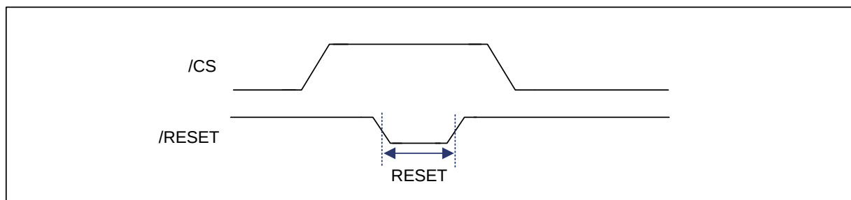
Figure 4-2 RESET Condition
