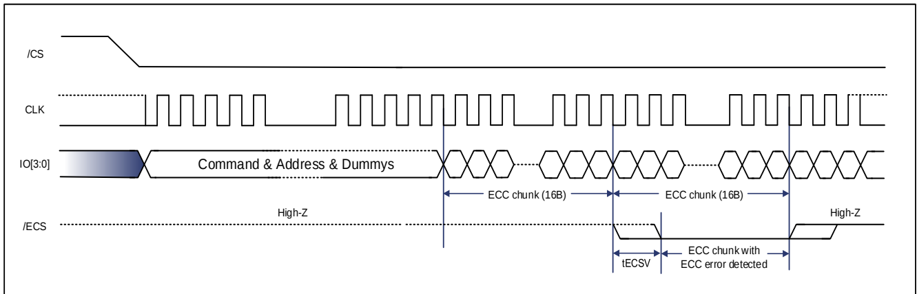
Figure 6-1. /ECS Timing
