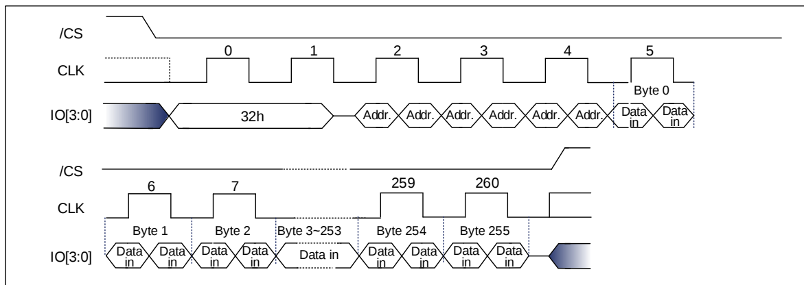
Figure 9-69 Quad Page Program Sequence Diagram (Quad DTR) [1]
