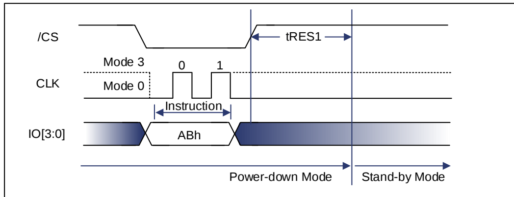
Figure 9-90 Release Power-Down Sequence Diagram (QPI & Quad DTR)
