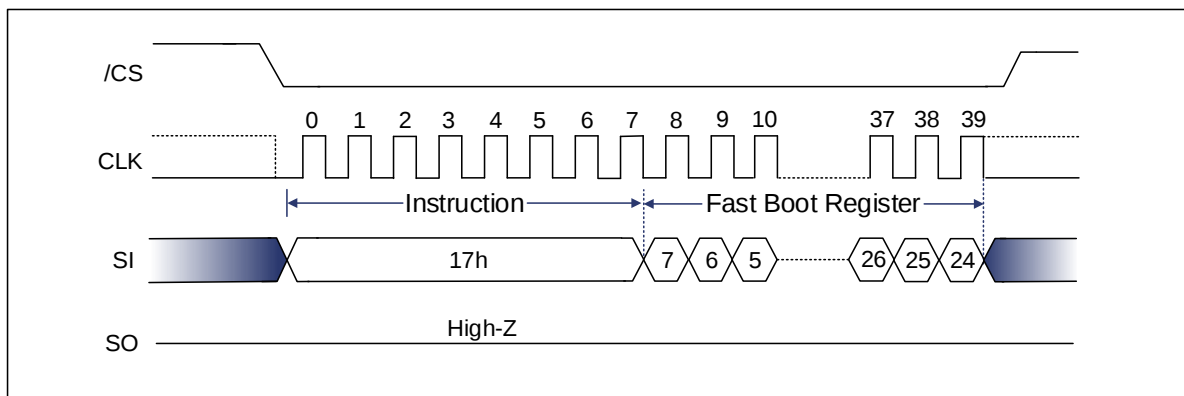
Figure 9-141 Write Fast Boot Register (WRFBR) Sequence
