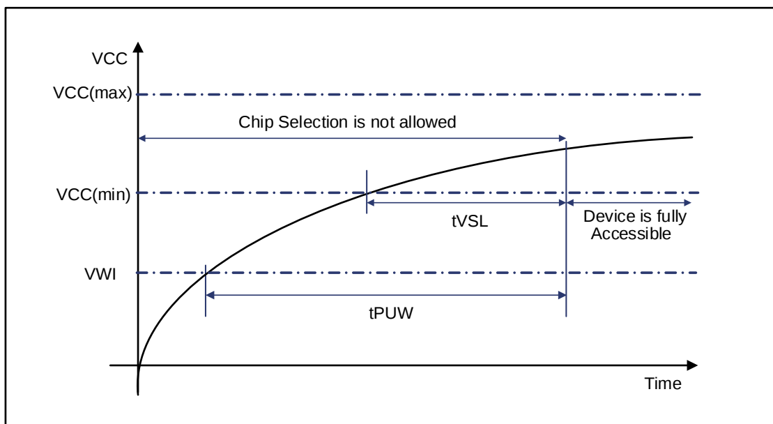
Figure 10-1 Power-Up Timing Sequence Diagram
