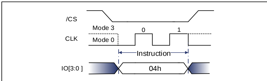
Figure 9-8 Write Disable Sequence Diagram (QPI and Quad DTR)
