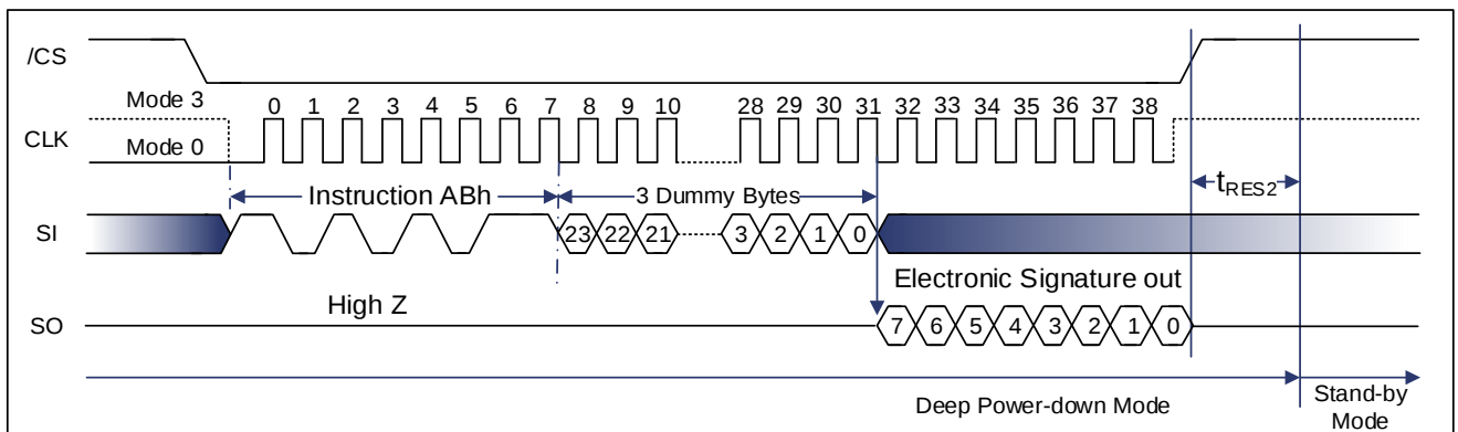
Figure 9-89 Release Power-Down/Read Device ID Sequence Diagram (SPI)
