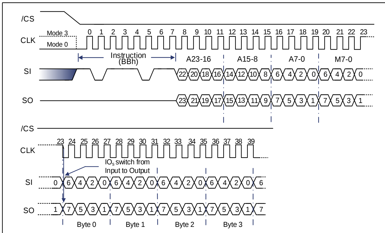
Figure 9-42 Dual I/O Fast Read Sequence Diagram ((M5-4) ≠ (1, 0))
