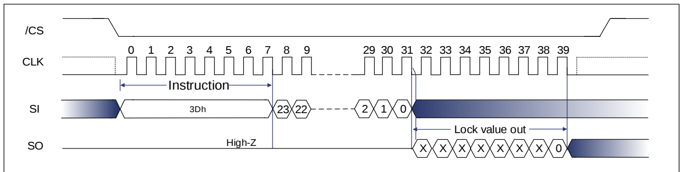
Figure 9-135 Read Individual Block/Sector lock command Sequence Diagram (SPI)
