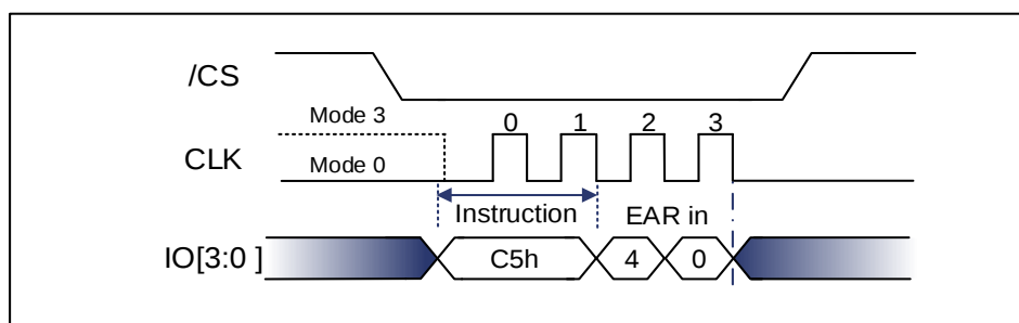
Figure 9-18 Write Extended Address Register Sequence Diagram (QPI)
