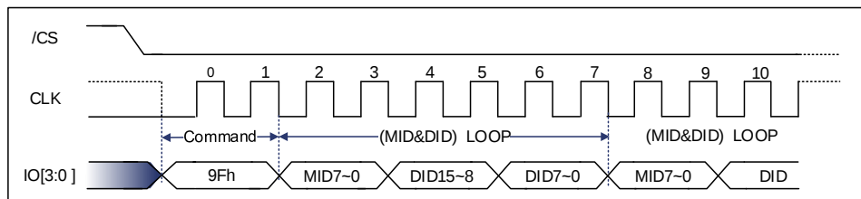
Figure 9-101 Read Identification ID Sequence Diagram (Quad DTR)
