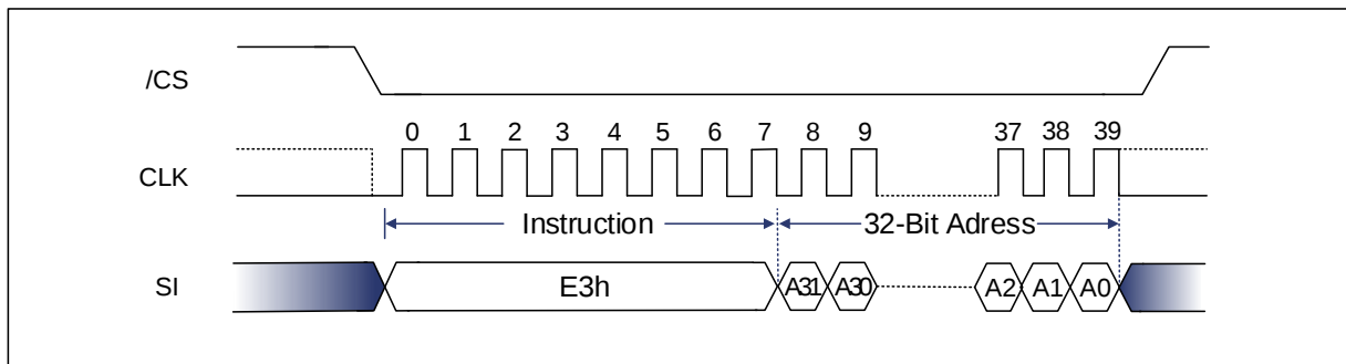
Figure 9-126 SPB Program (WRSPB) Sequence
