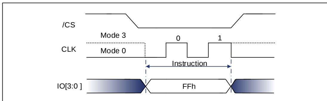
Figure 9-85 Disable QPI mode command Sequence Diagram (QPI and Quad DTR)
