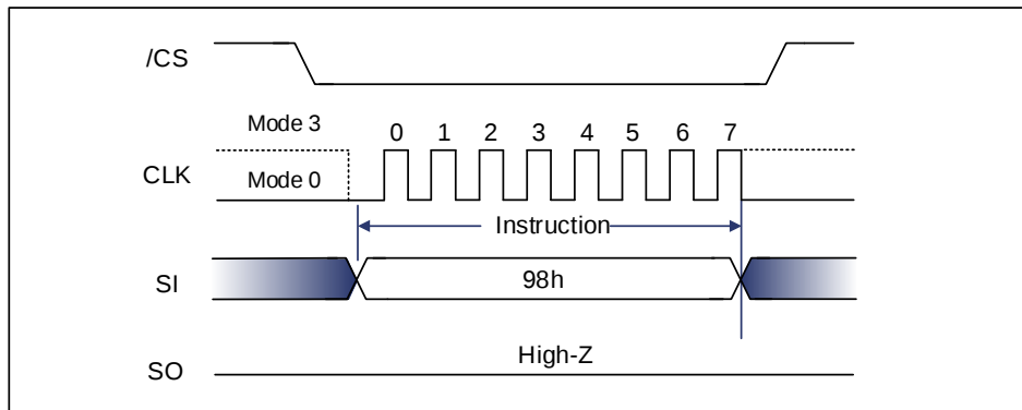
Figure 9-133 Global Block/Sector Unlock Sequence Diagram (SPI)
