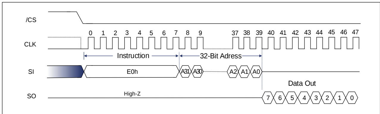
Figure 9-127 Read DPB Register (RDDPB) Sequence
