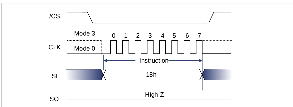
Figure 9-142 Erase Fast Boot Register (ESFBR) Sequence
