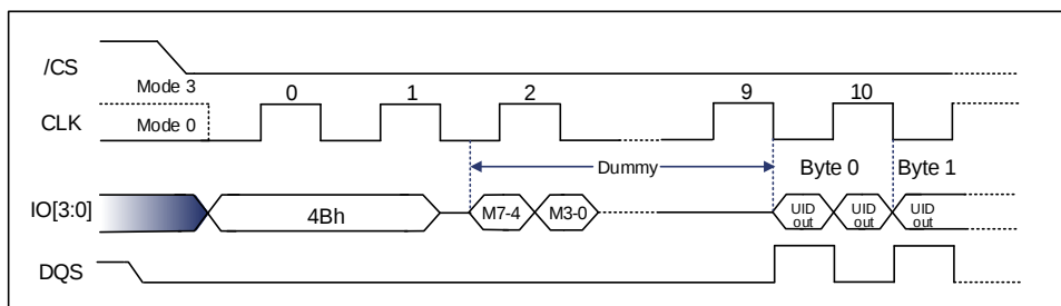
Figure 9-98 Read Unique ID Sequence Diagram (Quad DTR) [1]
