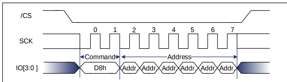
Figure 9-79 64KB Block Erase Sequence Diagram (QPI) [1]
