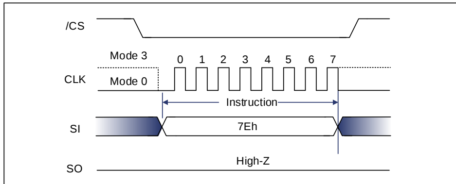
Figure 9-132 Global Block/Sector Lock Sequence Diagram (SPI)
