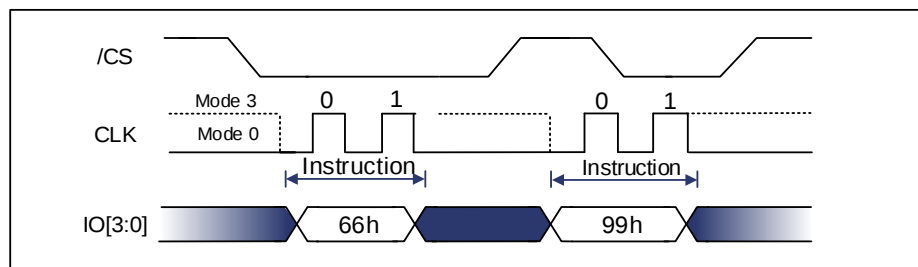
Figure 9-116 Enable Reset and Reset Command Sequence Diagram (QPI and Quad DTR)
