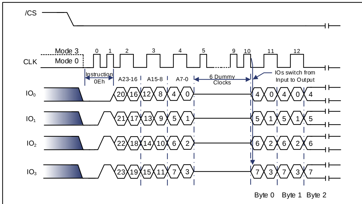
Figure 9-59 DTR Burst Read with Wrap Instruction (QPI Mode)
