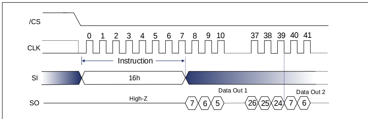
Figure 9-140 Read Fast Boot Register (RDFBR) Sequence
