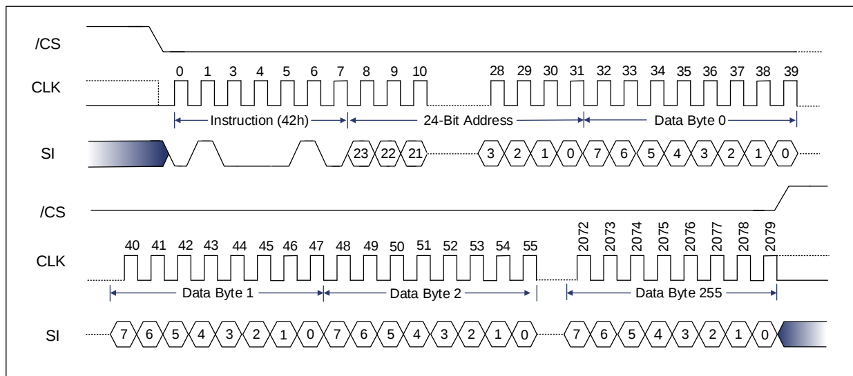
Figure 9-109 Program Security Registers Command Sequence Diagram (SPI) [1]
