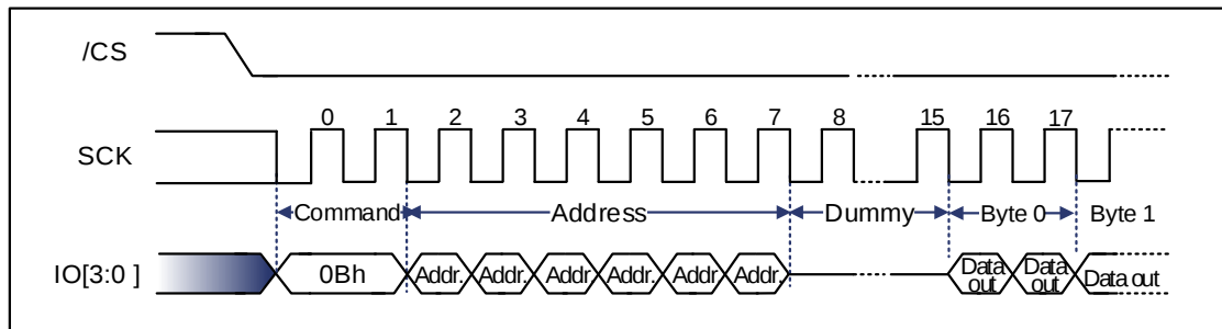
Figure 9-34 Read Data Bytes at Higher Speed Sequence Diagram (QPI) [1]
