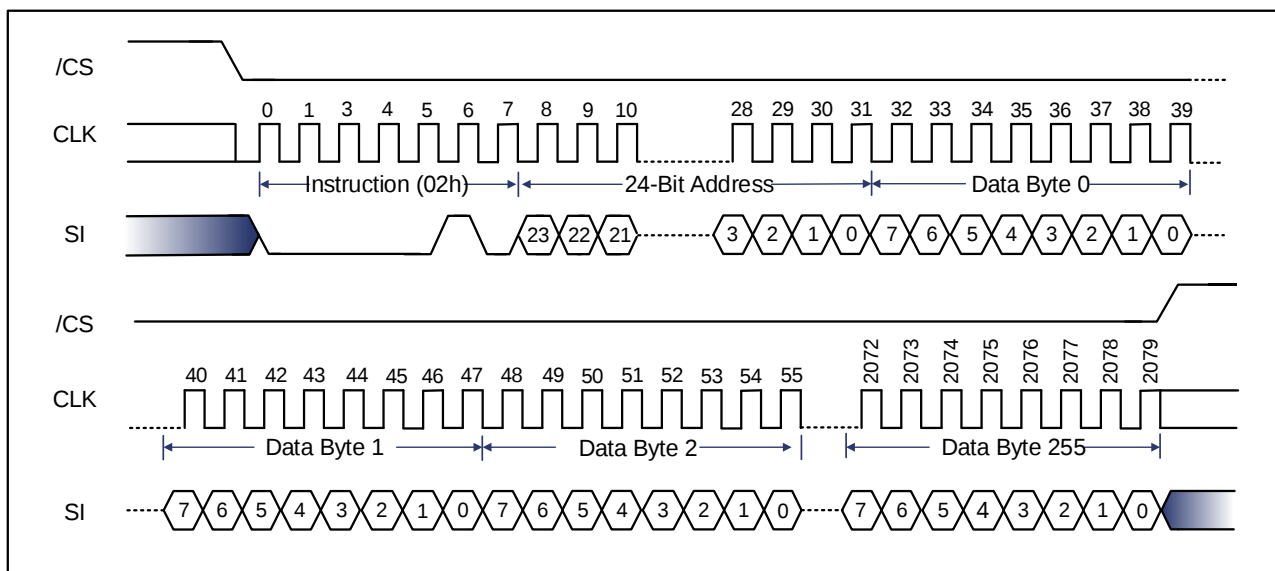
Figure 9-64 Page Program Sequence Diagram (SPI) [1]
