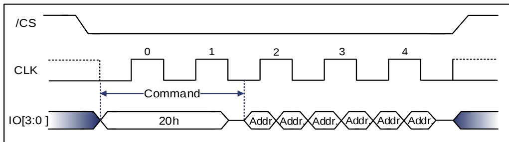
Figure 9-75 Sector Erase Sequence Diagram (Quad DTR) [1]
