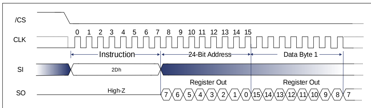
Figure 9-122 Read Lock Register (RDLR) Sequence (SPI Mode)
