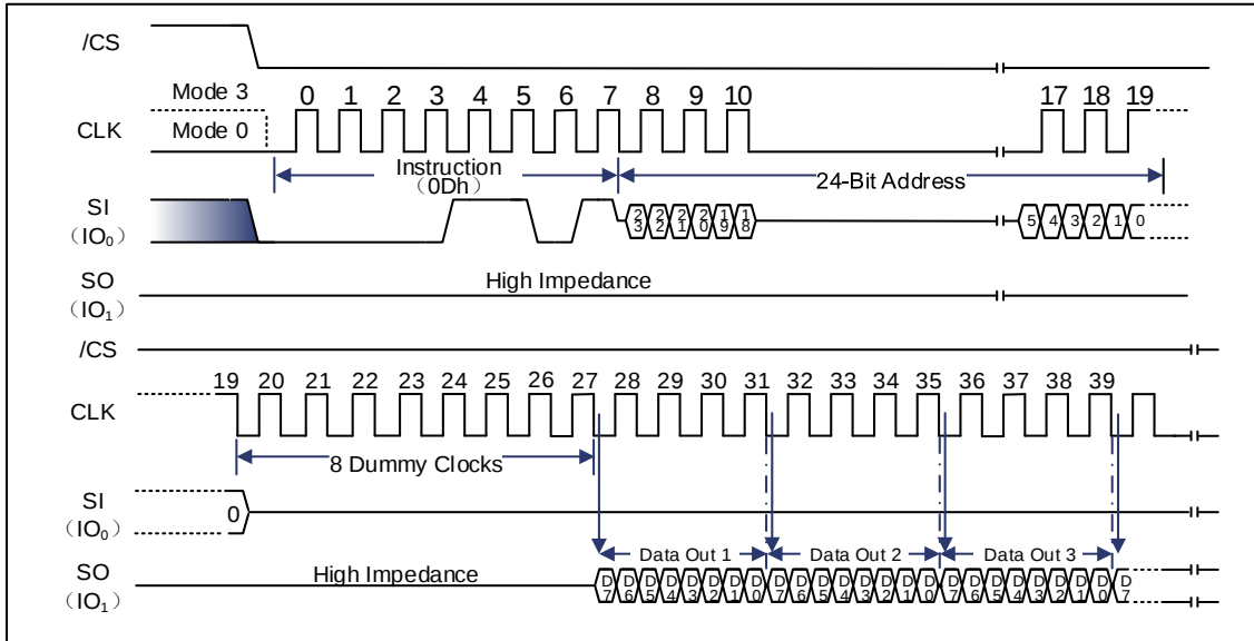
Figure 9-36 DTR Fast Read Instruction (SPI Mode)
