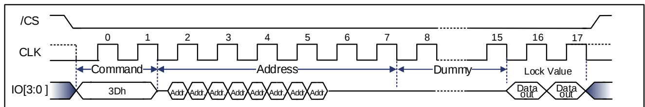
Figure 9-136 Read Individual Block/Sector lock command Sequence Diagram (QPI)
