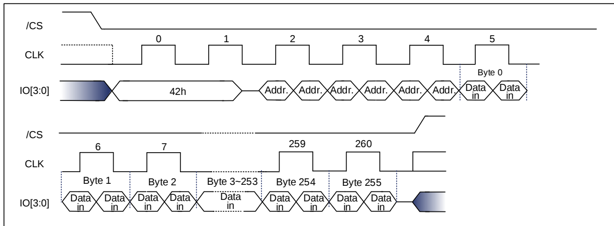
Figure 9-111 Program Security Registers Command Sequence Diagram (Quad DTR) [1]
