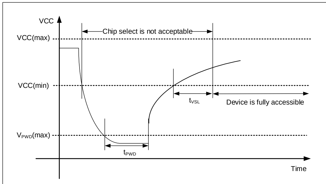
Figure 58C. Power-Down Requirement
