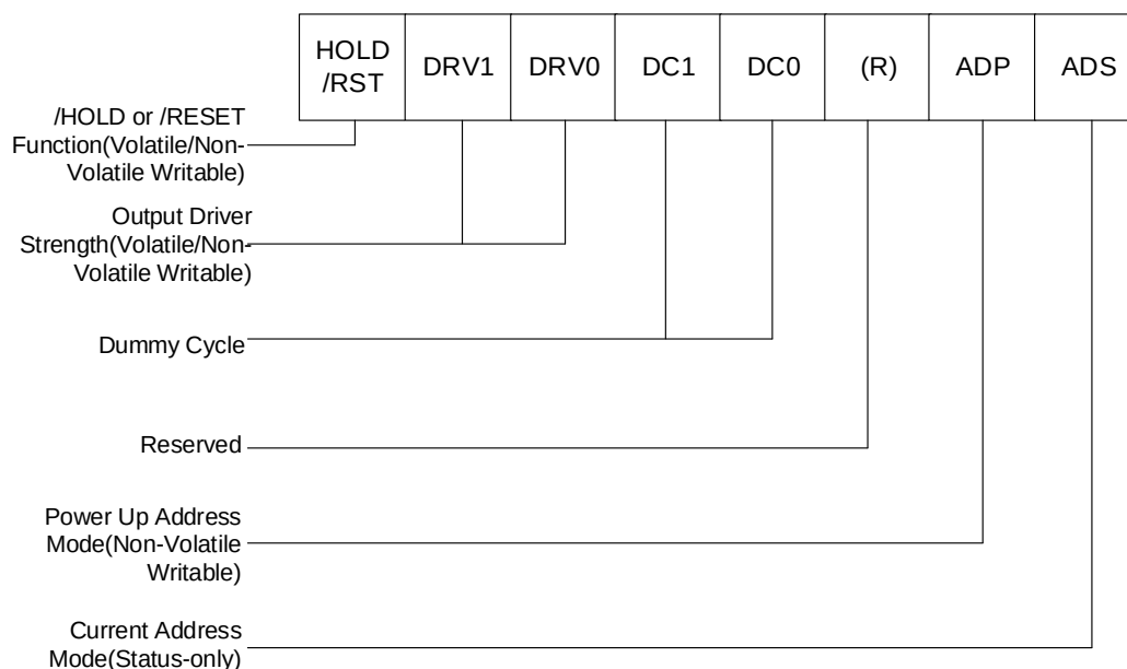
Figure 4c. Status Register-3
