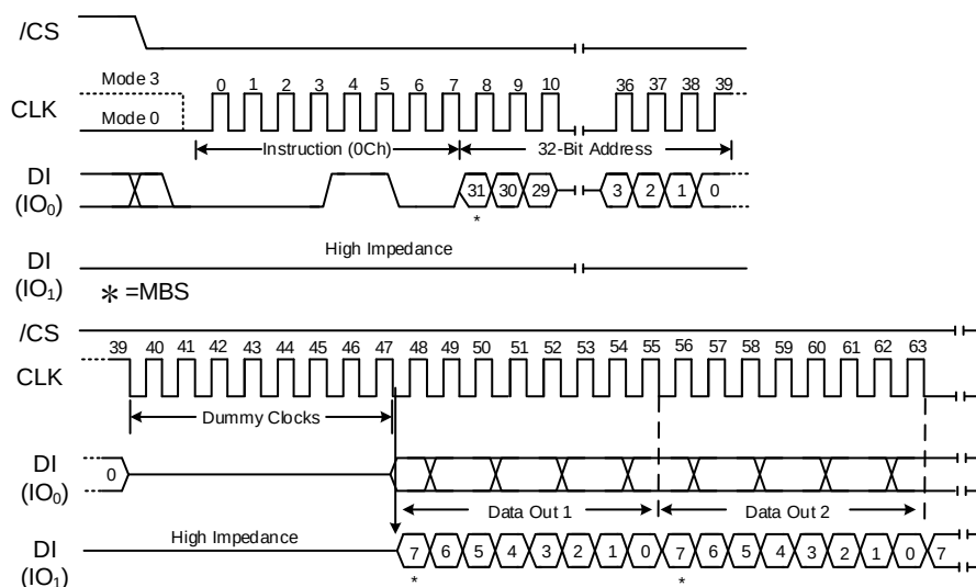
Figure 17. Fast Read with 4-Byte Address Instruction
