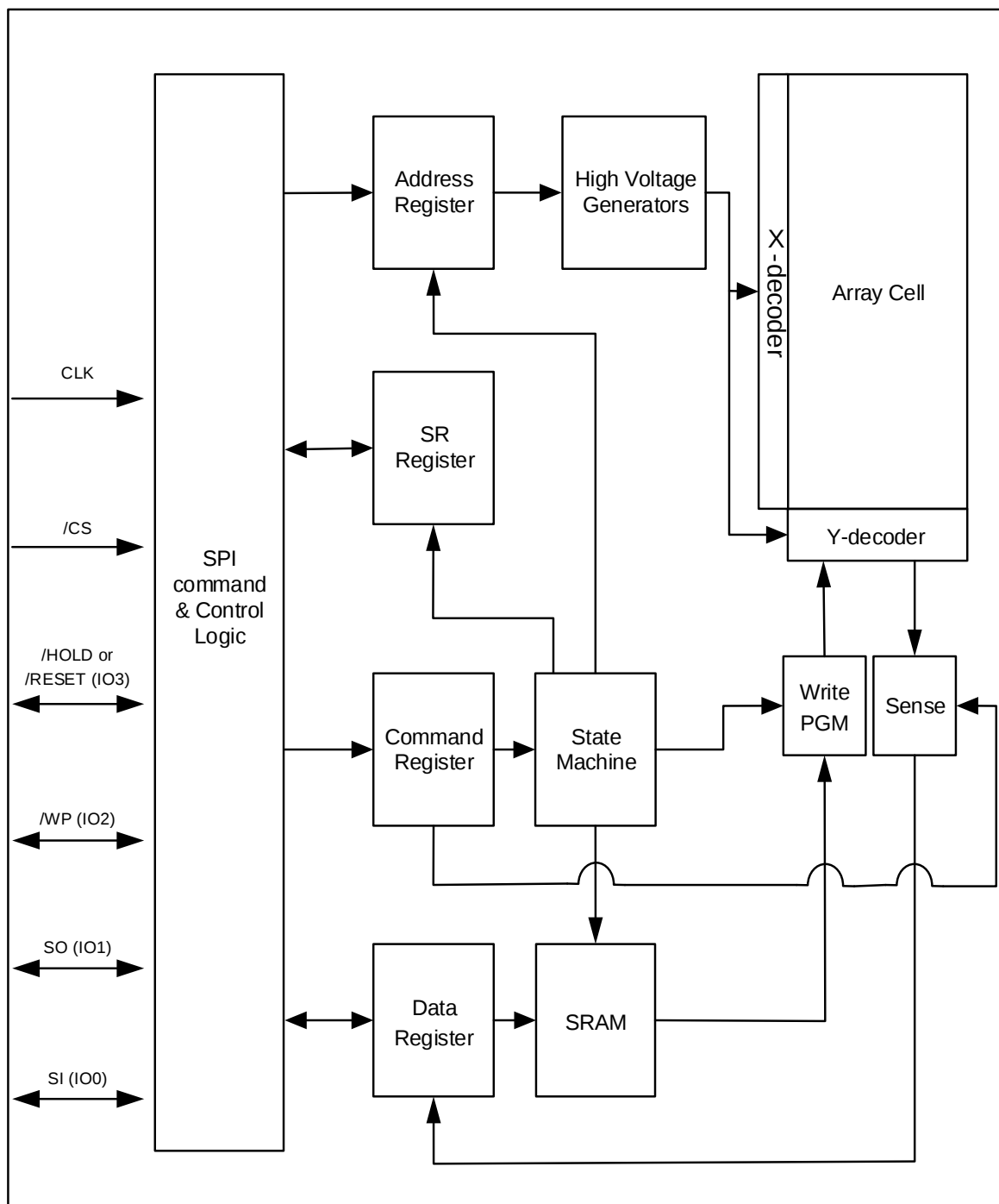
Figure 4-1 XM25QU512D Serial Flash Memory Block Diagram
