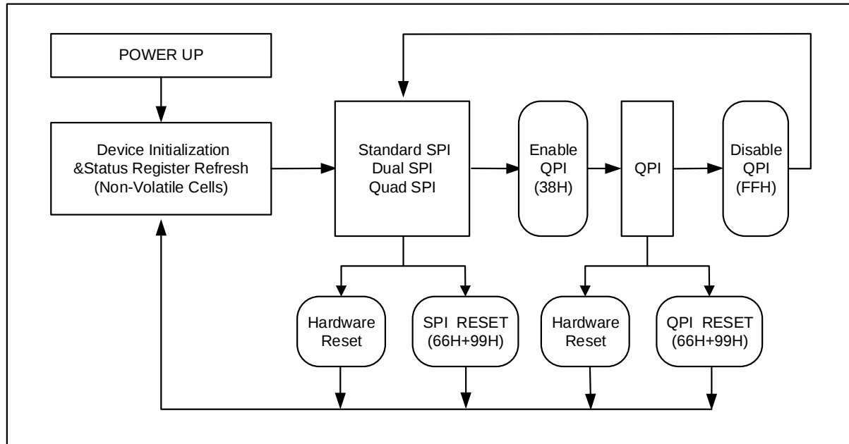
Figure 7-1 XM25QU512D Serial Flash Memory Operation Diagram
