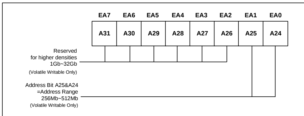
Figure 8-4 Extended Address Register
