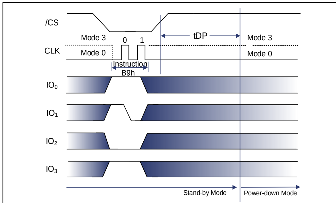
Figure 9-61 Deep Power-down Instruction (QPI Mode)
