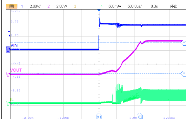
V_{IN}=3.7V V_{OUT}=5V R_{OUT}=25\Omega Figure13.Startup by V_{IN}
