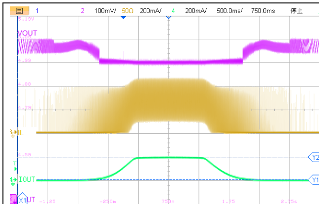
Figure23.Load Transient
