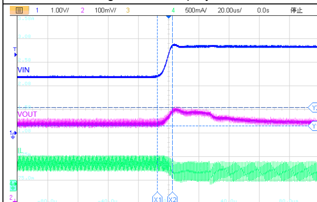
V_{IN}=2.4V to 3.7V V_{OUT}=5V I_{OUT}=200mA Figure15.Line Transient
