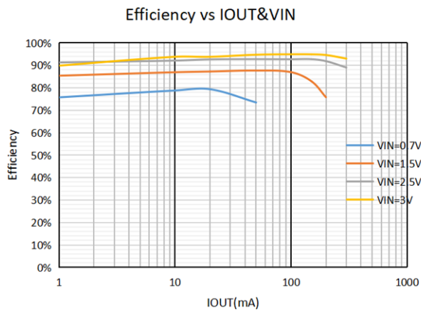
Figure1.Load Efficiency with Different Input
