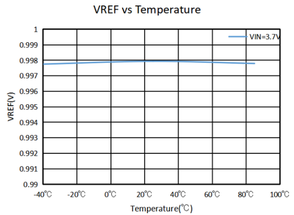
ET82099, V IN =3.7V T A =-40°C~85°C Figure 8. Reference Voltage vs Temperature
