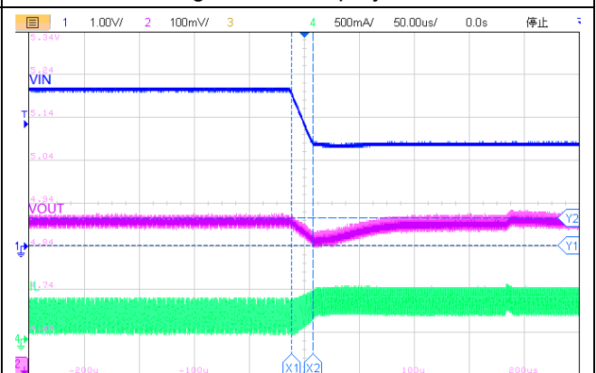
V_{IN}=3.7V to 2.4V V_{OUT}=5V I_{OUT}=200mA Figure16.Line Transient
