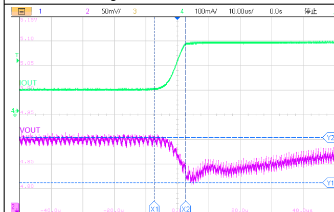
Figure19.Load Transient
