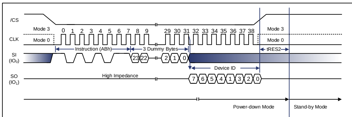
Figure 9-68 Release Power-down / Device ID Instruction (SPI Mode)
