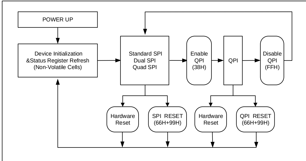
Figure 7-1 XM25QH512D Serial Flash Memory Operation Diagram
