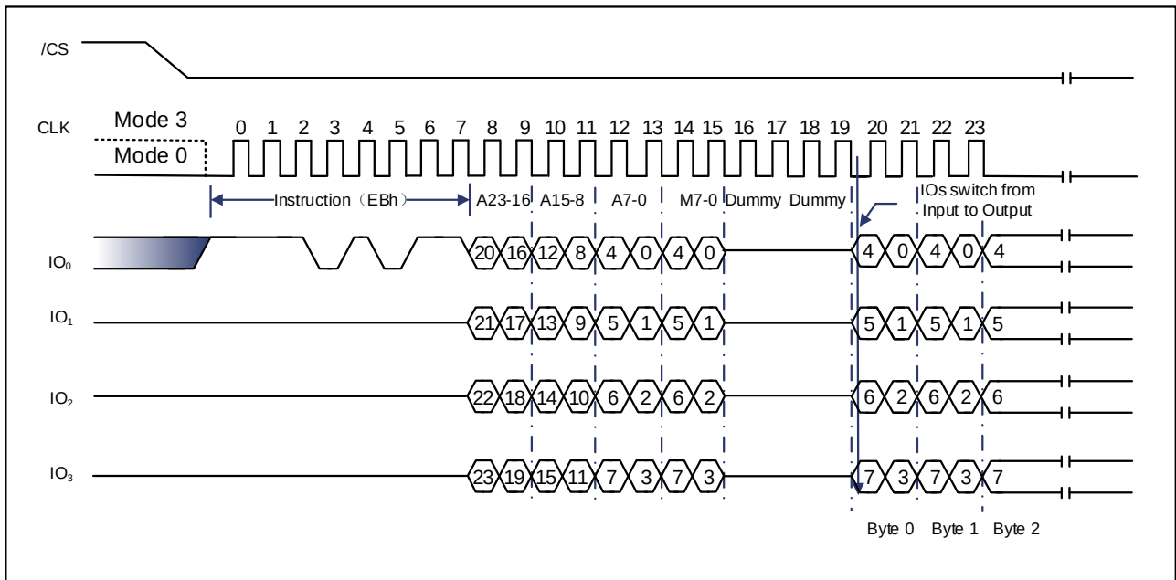
Figure 9-33 Fast Read Quad I/O Instruction (Initial instruction or previous M5-4≠10, SPI Mode)
