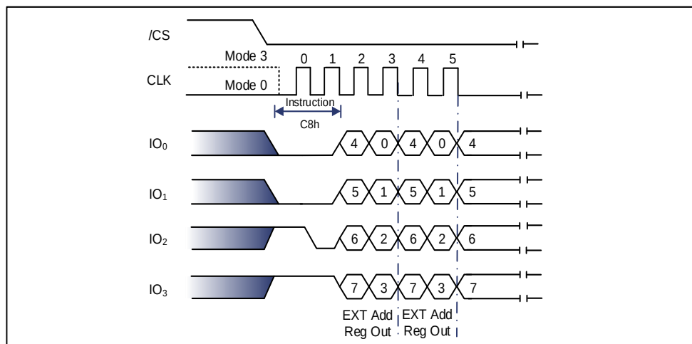
Figure 9-11 Read Extended Address Register Instruction (QPI Mode)
