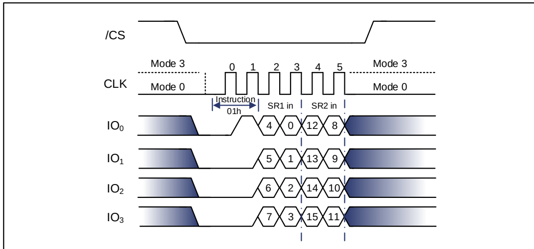
Figure 9-9 Write Status Register-1/2 Instruction (QPI Mode)
