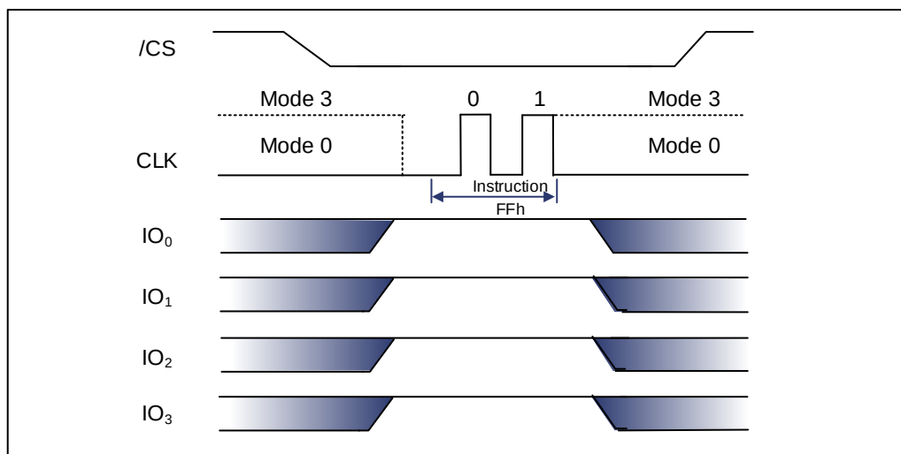
Figure 9-84 Exit QPI Instruction (QPI Mode only)
