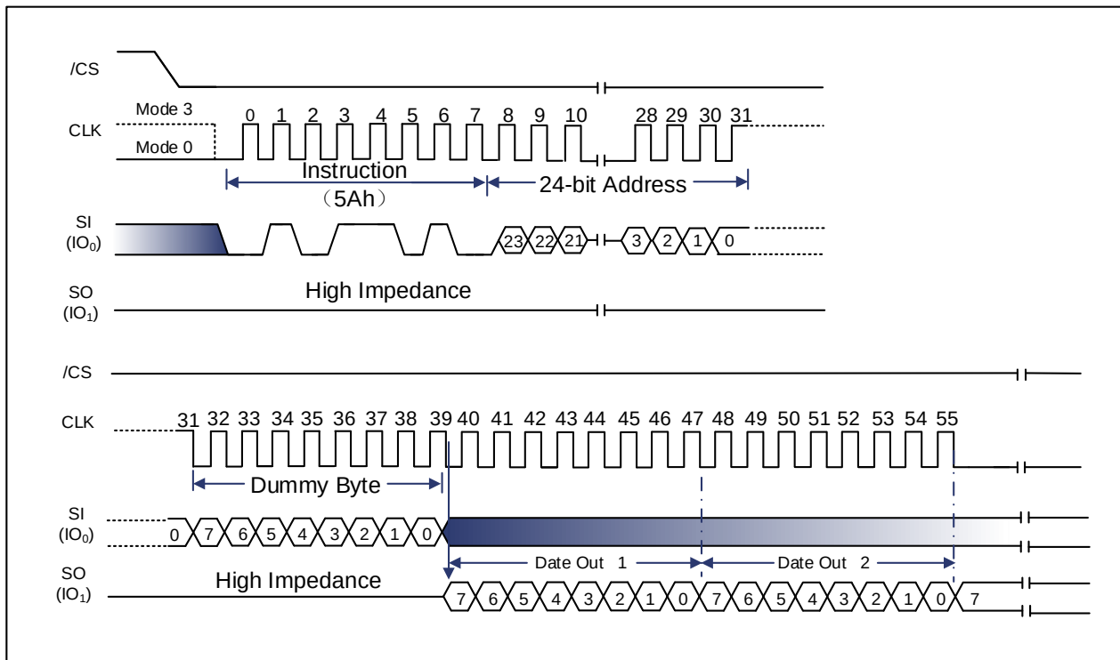
Figure 9-76 Read SFDP Register Instruction Sequence Diagram(Only SPI Mode)
