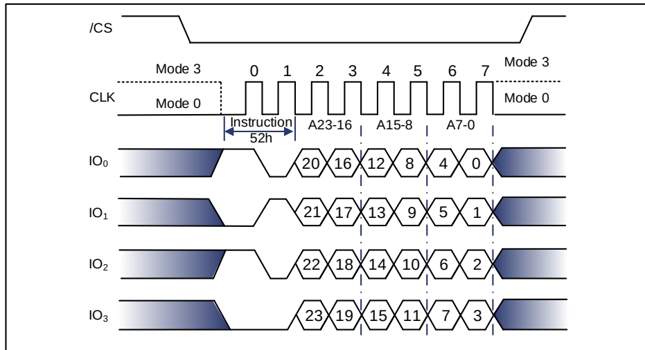
Figure 9-52 32KB Block Erase Instruction (QPI Mode)
