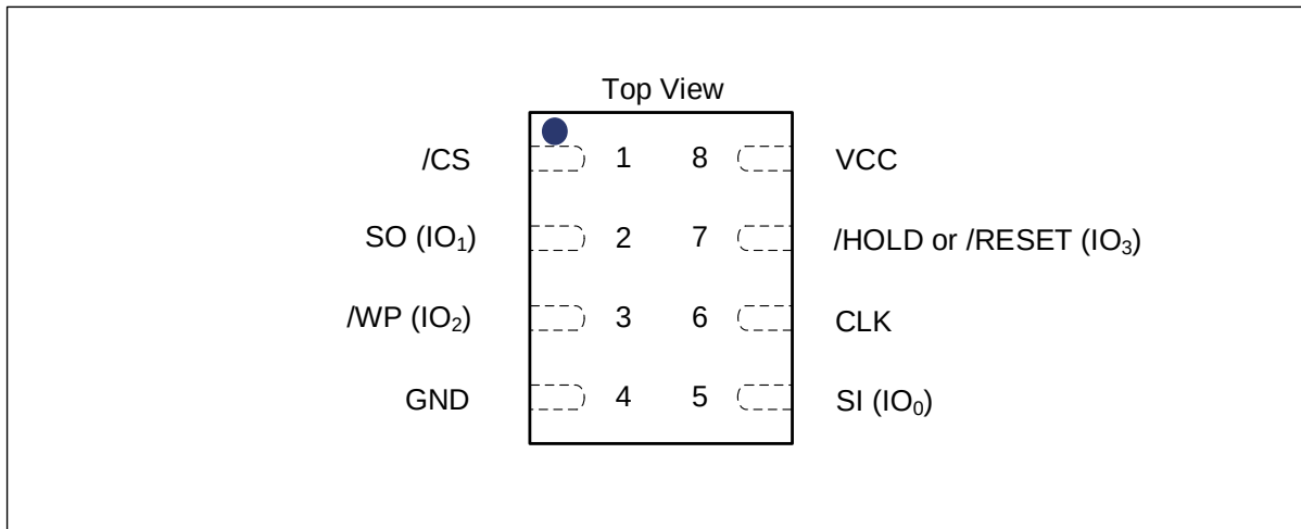
Figure 5-2 8-pin WSON (Package Code X)
