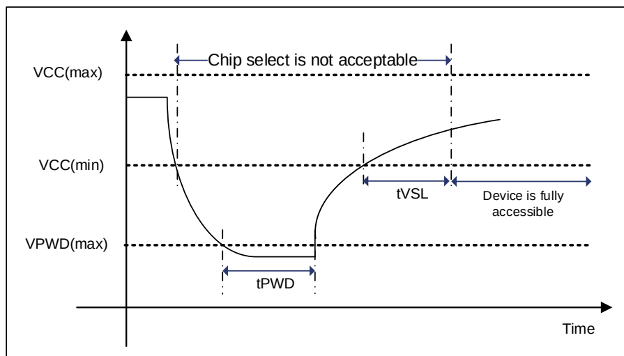
Figure 10-4 Power-Down and Power-up Requirement
