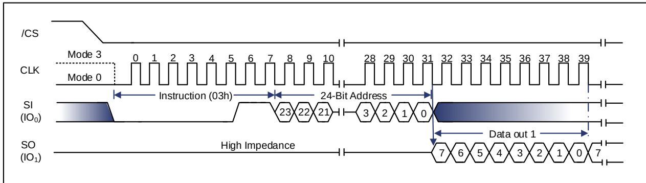
Figure 9-16 Read Data Instruction (SPI Mode only)
