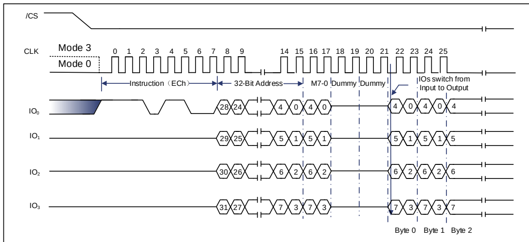
Figure 9-35 Fast Read Quad I/O Instruction (Initial instruction or previous M5-4≠10, SPI Mode)
