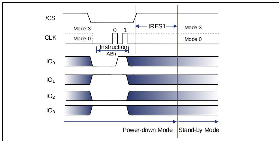
Figure 9-67 Release Power-down Instruction (QPI Mode)
