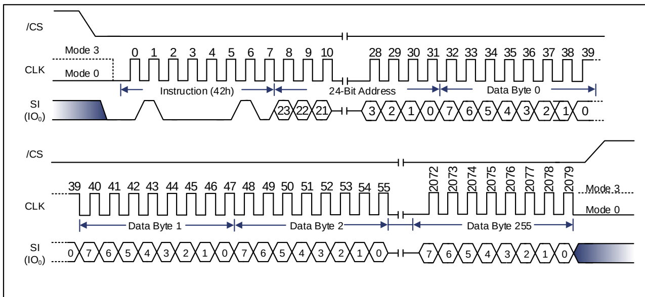
Figure 9-78 Program Security Registers Instruction (SPI Mode only) 32-Bit Address is required when the device is operating in 4-Byte Address Mode
