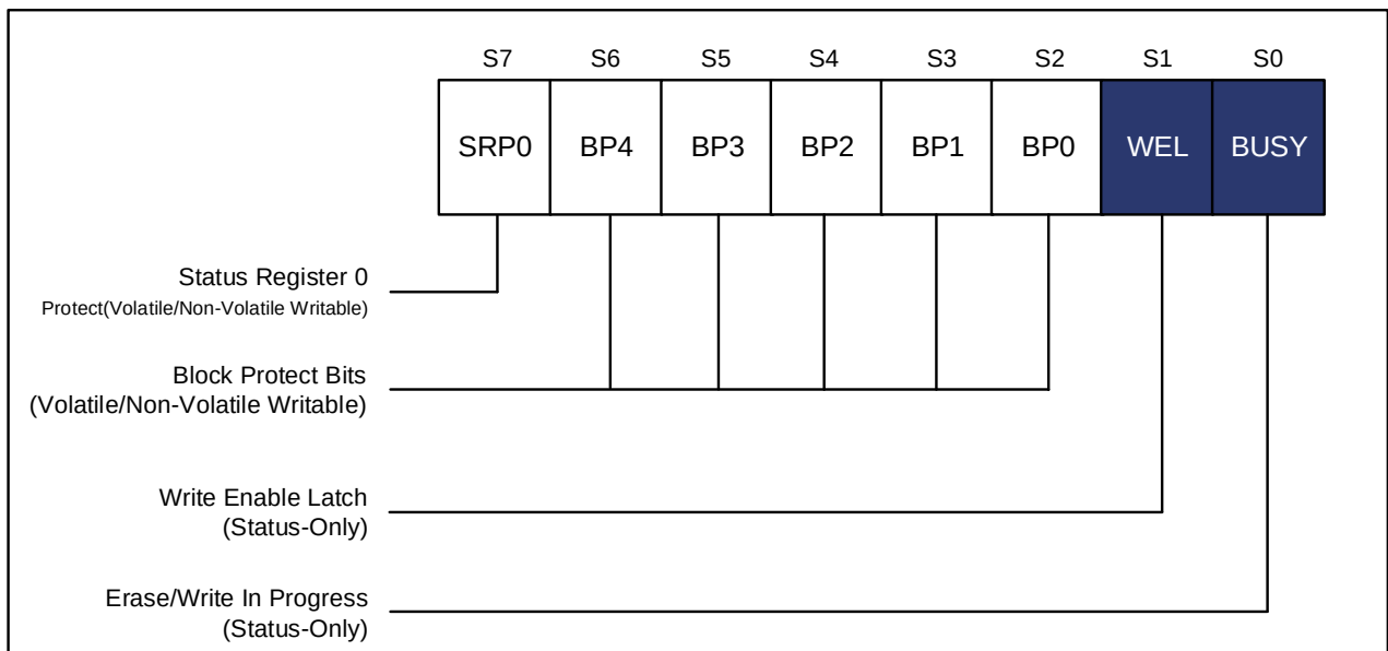
Figure 8-1 Status Register-1
