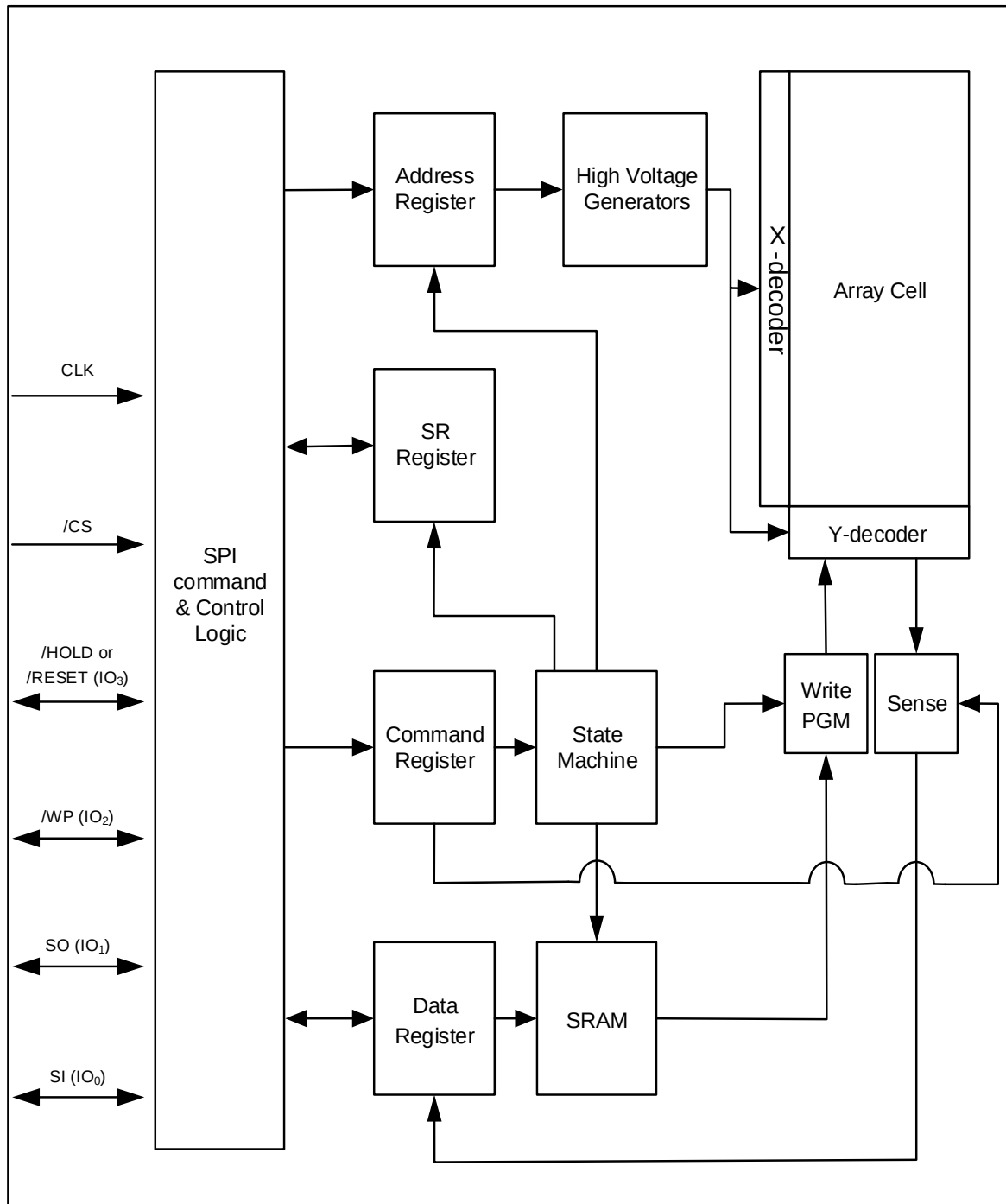
Figure 4-1 XM25QH512D Serial Flash Memory Block Diagram
