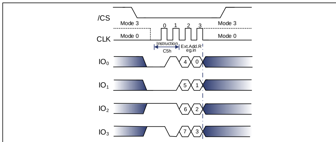
Figure 9-13 Write Extended Address Register Instruction (SPI Mode)
