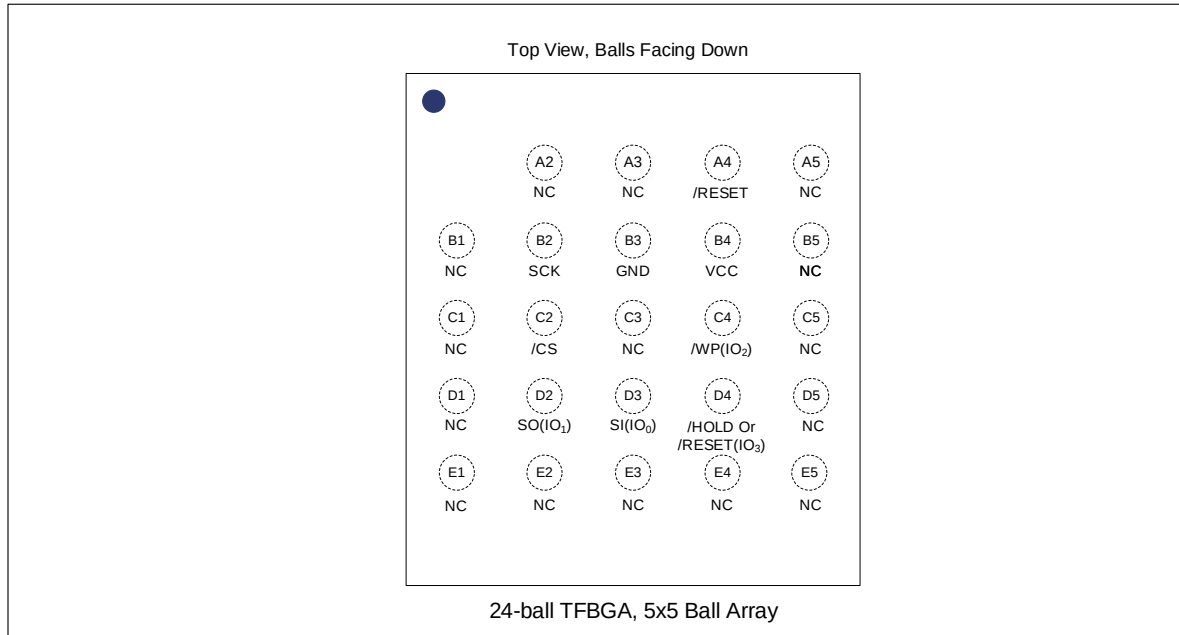
Figure 5-3 24-ball TFBGA 8x6-mm, 6x4 and 5x5 (Package Code B2)
