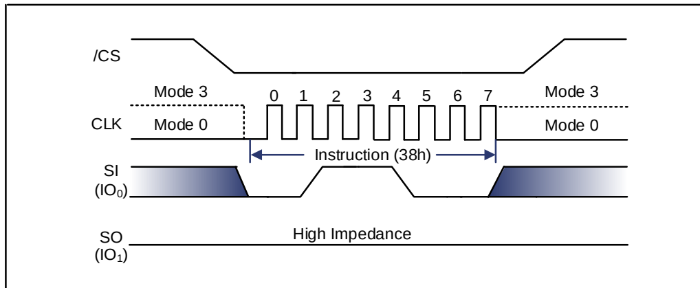
Figure 9-83 Enter QPI Instruction (SPI Mode only)
