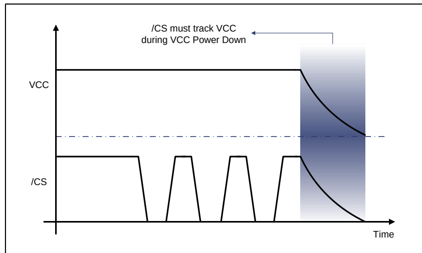
Figure 10-3 Power-Down Timing
