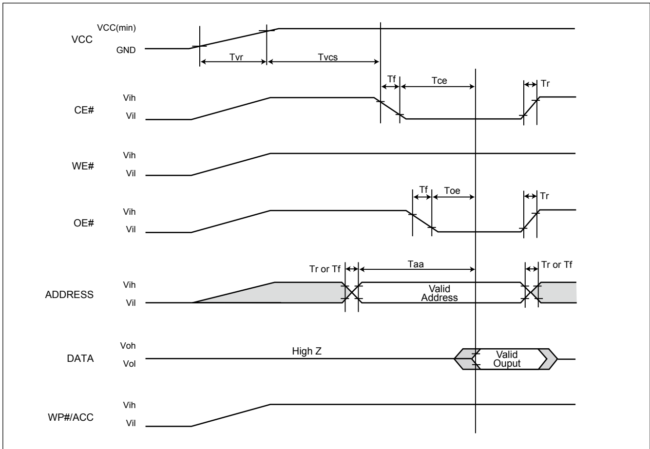
Figure 30. AC Timing at Device Power-Up
