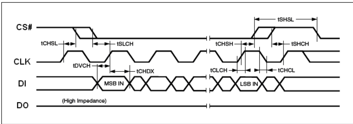
Figure 50. Input Timing
