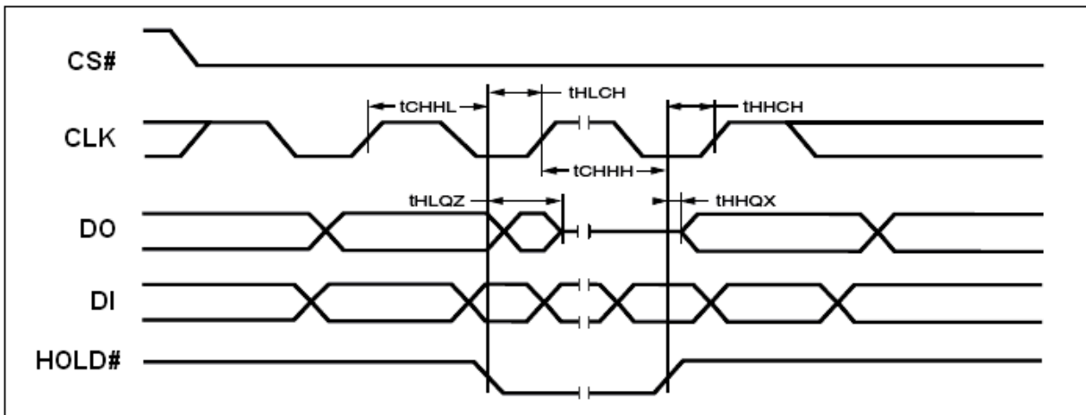
Figure 51. Hold Timing
