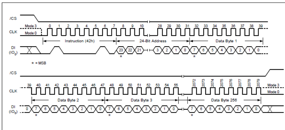
Figure 43. Program OTP array
