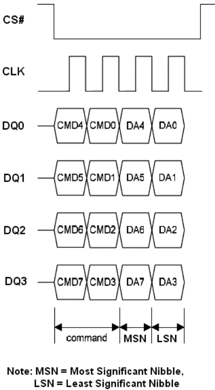
Figure 28.1 Write Status Register 3 Instruction Sequence Diagram in QPI mode
