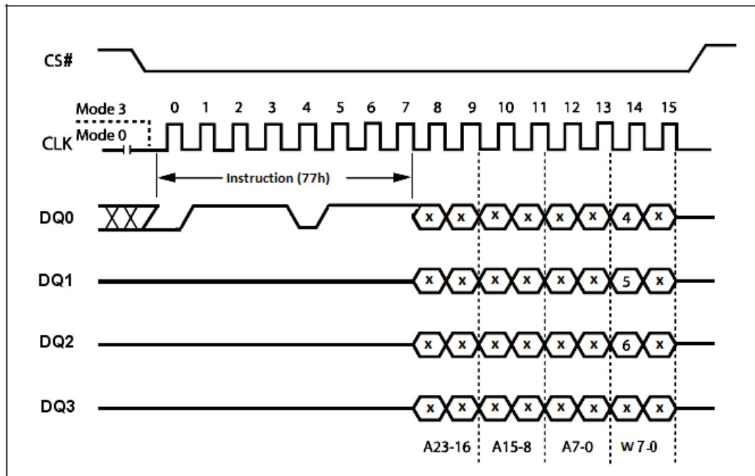
Set Burst with Wrap Sequence Diagram
