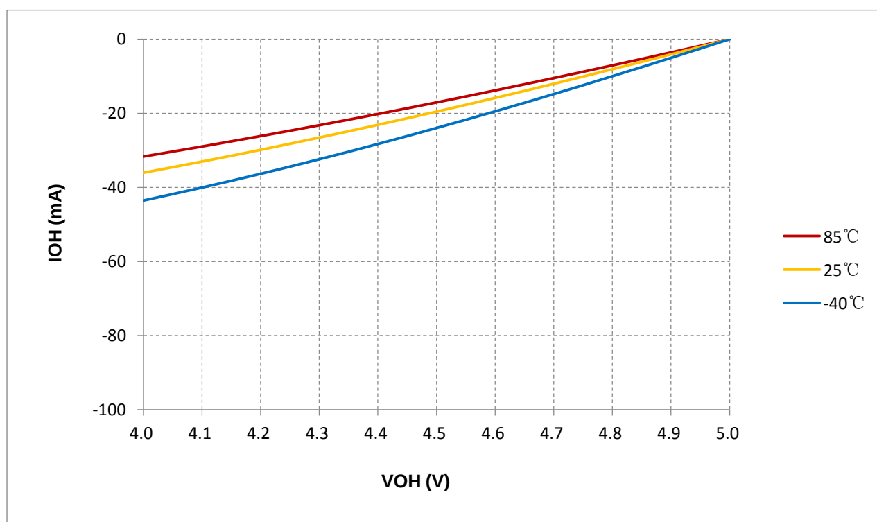
图 19-8 I_{OH} vs. V_{OH} @L2 = -18mA , V_{DD} = 5V
