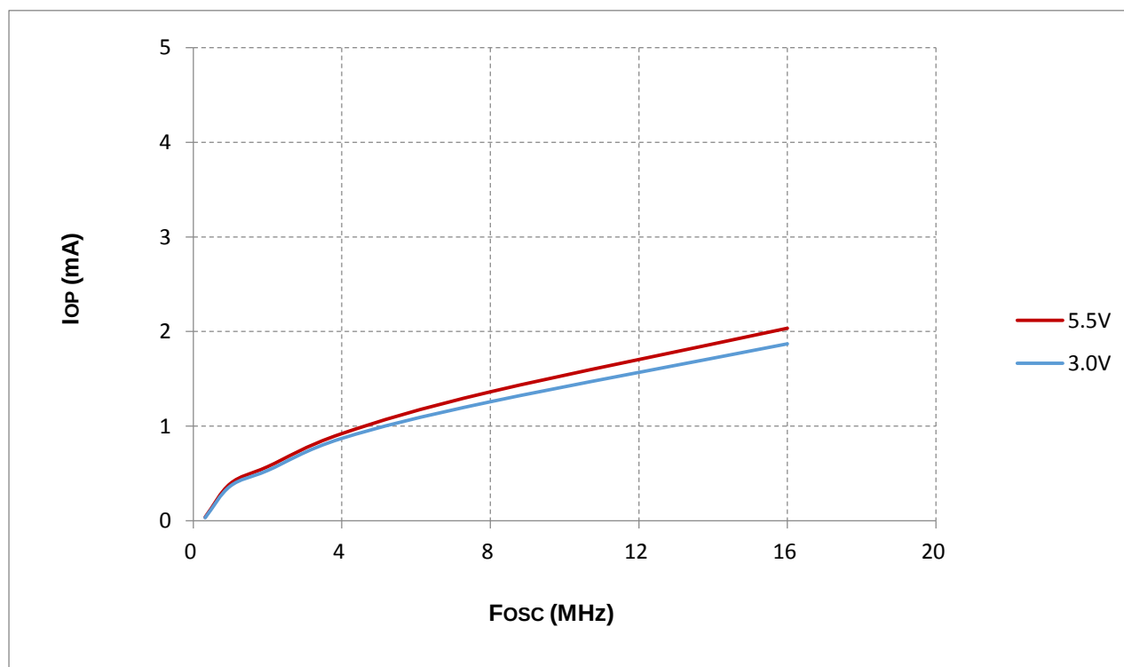
图 19-4 I_{DD} vs. Frequency (2T, T_A = 25^\circ\text{C} )
