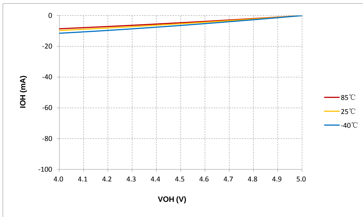
图 19-7 I_{OH} vs. V_{OH} @L1 = -5mA , V_{DD} = 5V
