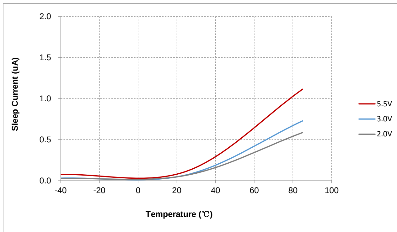
图 19-5 Sleep Current ( I_{SB} ) vs. Temperature
