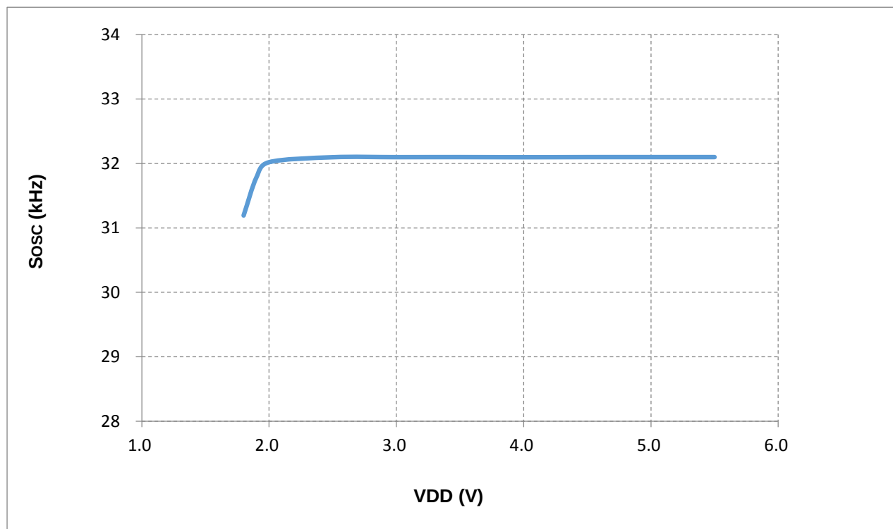
图 19-3 LIRC vs. V_{DD} ( T_A = 25^\circ\text{C} )
