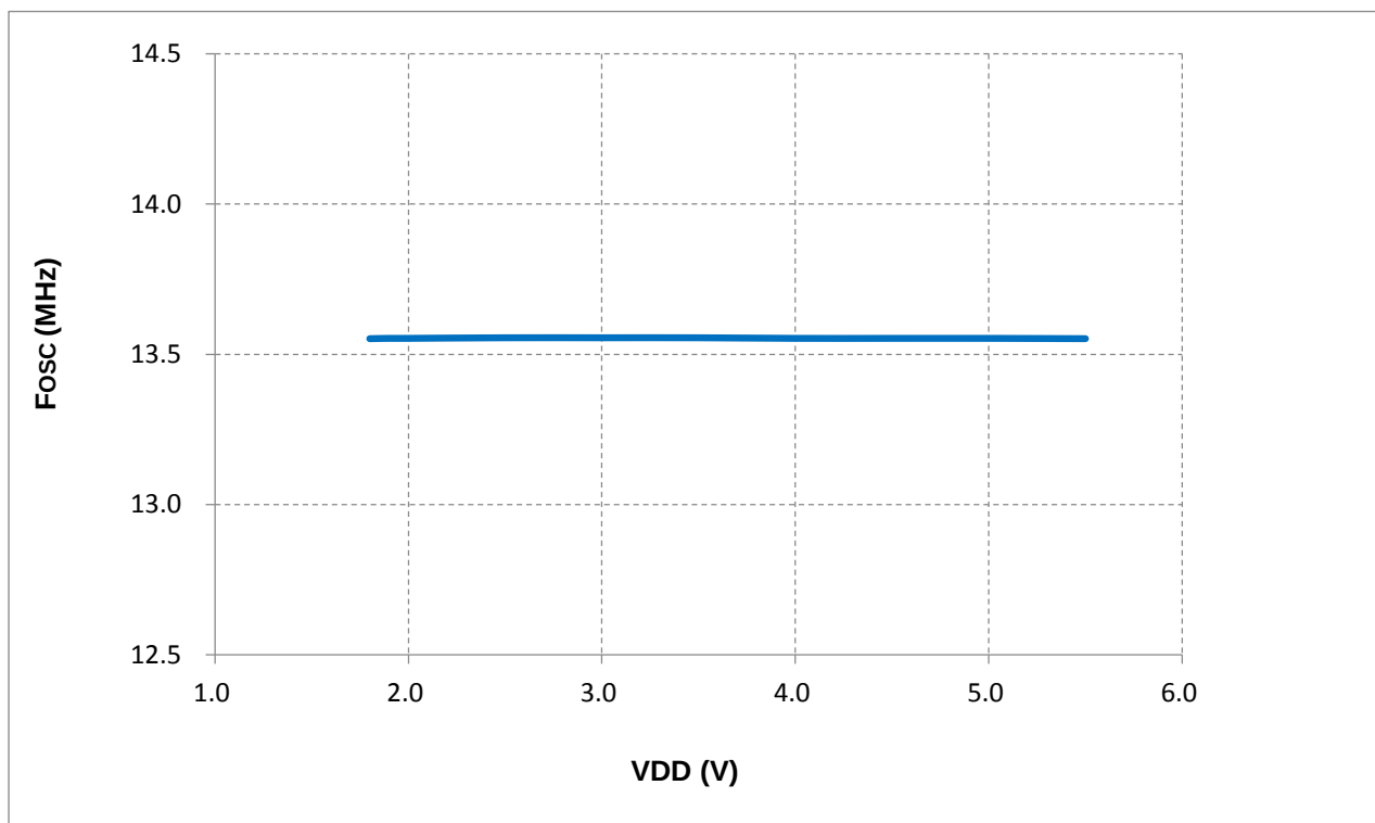
图 19-2 HIRC (13.56M) vs. V_{DD} ( T_A = 25^\circ\text{C} )
