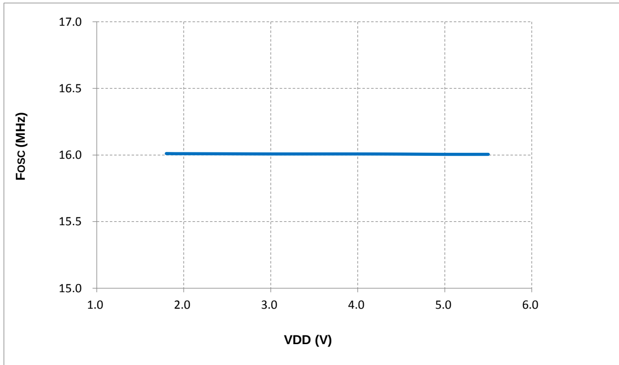
图 19-1 HIRC (16M) vs. V_{DD} ( T_A = 25^\circ\text{C} )
