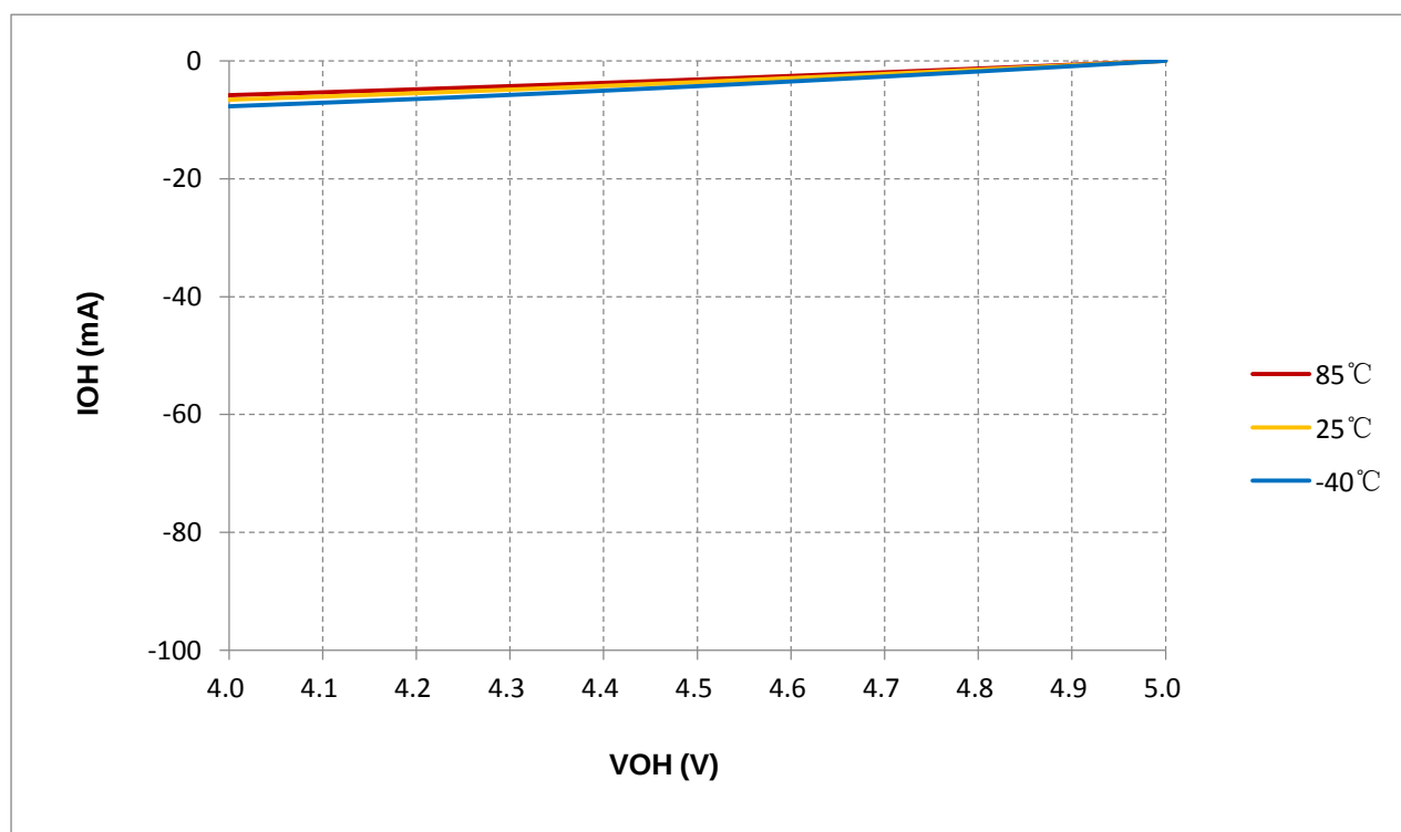
图 19-6 I_{OH} vs. V_{OH} @ L0 = -3mA , V_{DD} = 5V
