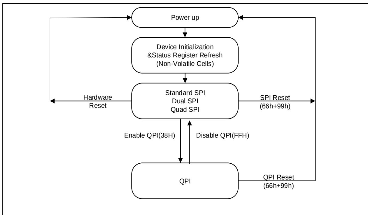
Figure 3. XM25QW16C Serial Flash Memory Operation Diagram
