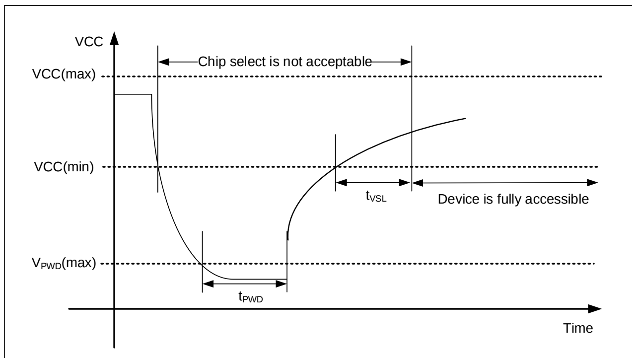
Figure 45C. Power-Down Requirement
