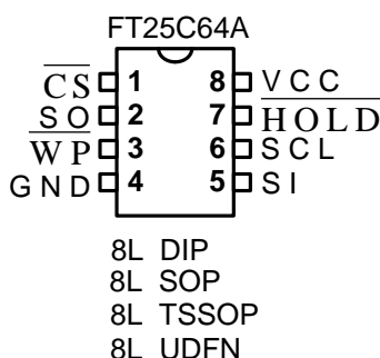
Figure 1: Packaging Types
