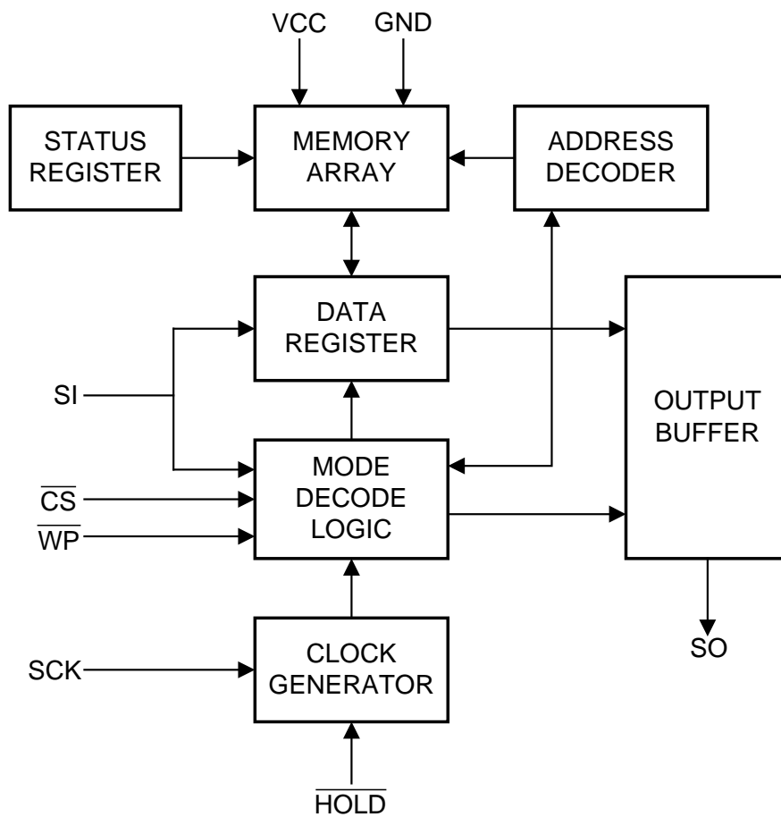
Figure 2: Block Diagram
