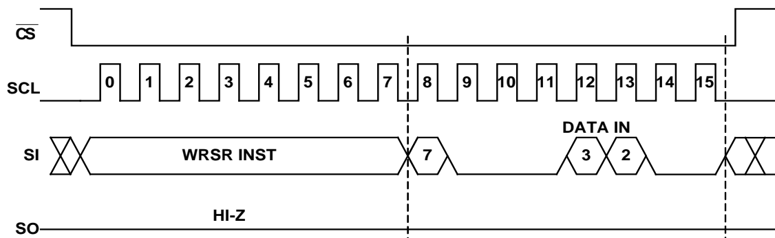
Figure 8: WRSR Timing
