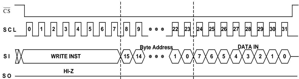
Figure 10: WRITE Timing
