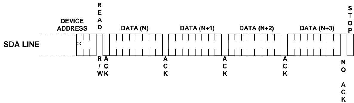
Figure 8: Sequential Read
