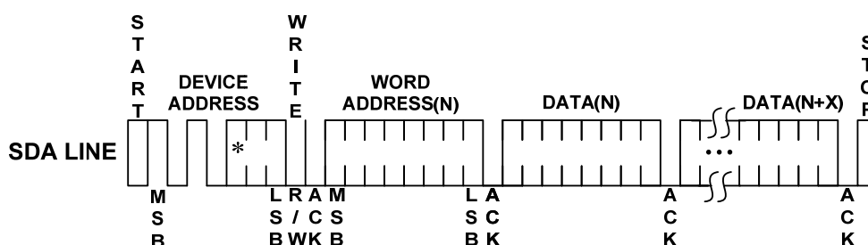
Figure 6: Page Write
