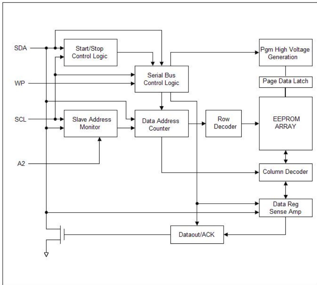
Figure 2: Block Diagram
