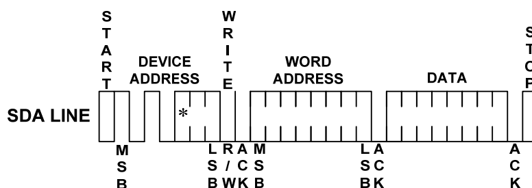
Figure 5: Byte Write
