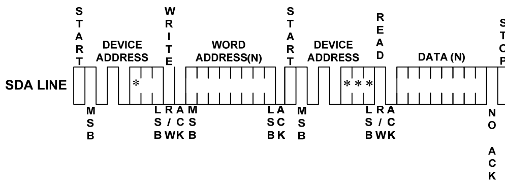
Figure 9: Random Read
