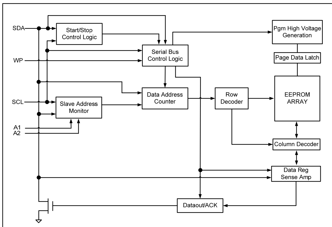
Figure 2: Block Diagram
