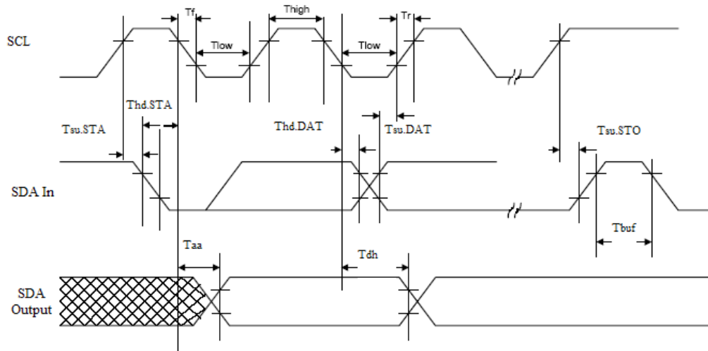
Figure 10: SCL and SDA Bus Timing
