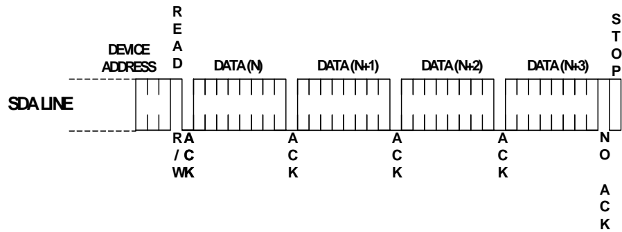
Figure 8: Sequential Read
