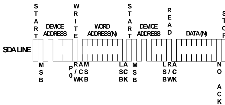
Figure 9: Random Read
