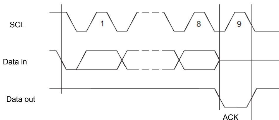
Figure 4: Timing diagram for output ACKNOWLEDGE
