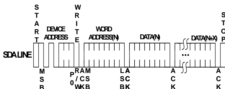
Figure 6: Page Write
