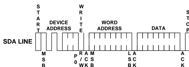
Figure 5: Byte Write
