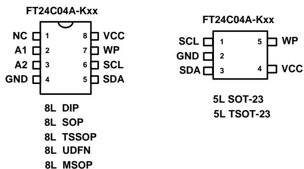
Figure 1: Package types
