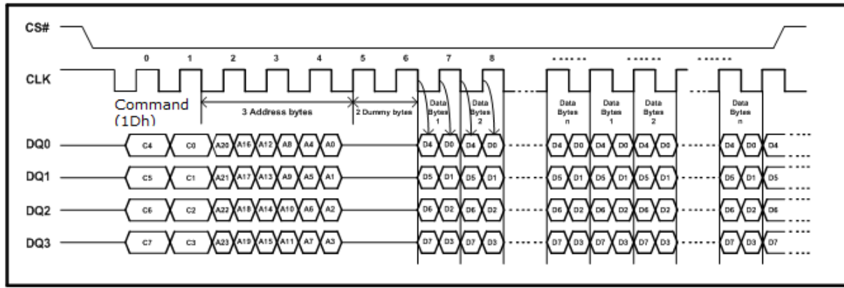
DDR Read Burst with Wrap Instruction Sequence Diagram in QPI mode
