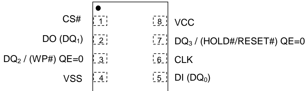
8 – LEAD USON / VDFN / WSON
