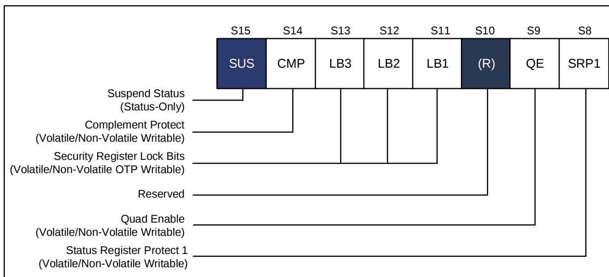
Figure 8-2 Status Register-2
