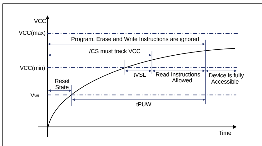
Figure 10-2 Power-up Timing and Voltage Levels
