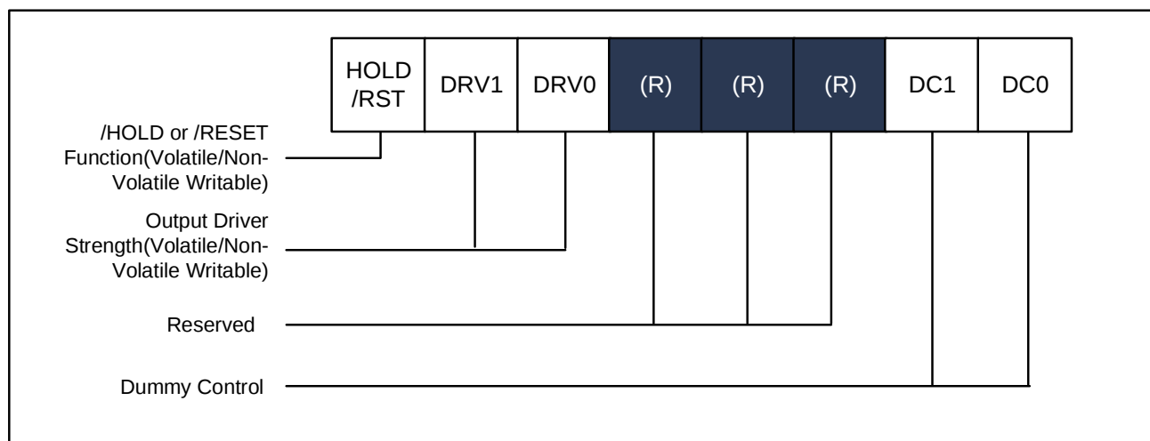
Figure 8-3 Status Register-3
