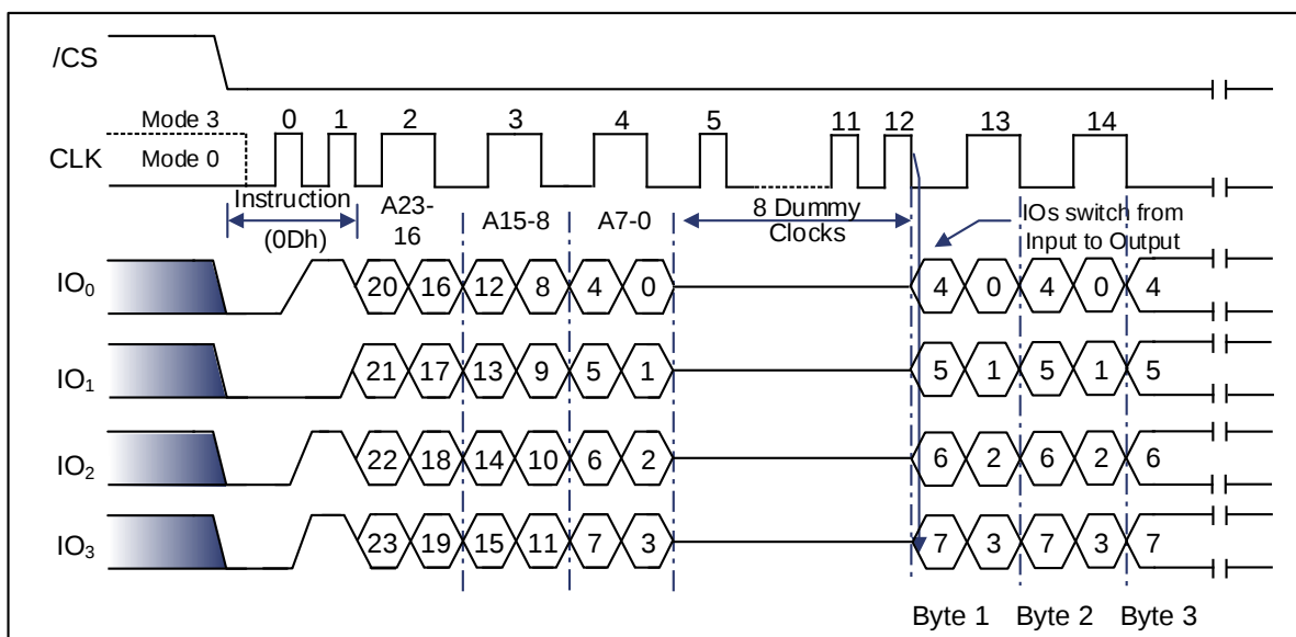
Figure 9-14 DTR Fast Read Instruction (QPI Mode)
