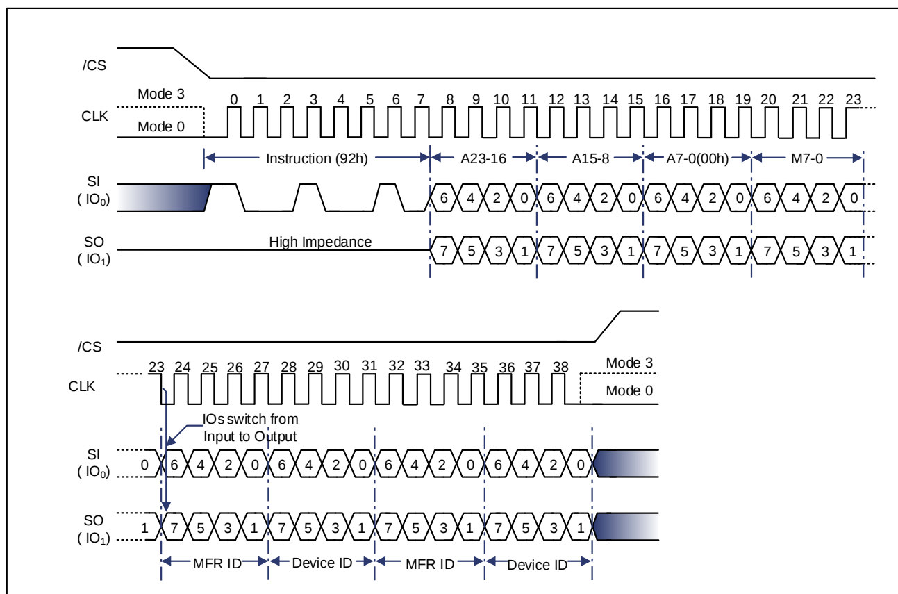
Figure 9-51 Read Manufacturer / Device ID Dual I/O Instruction (SPI Mode only)
