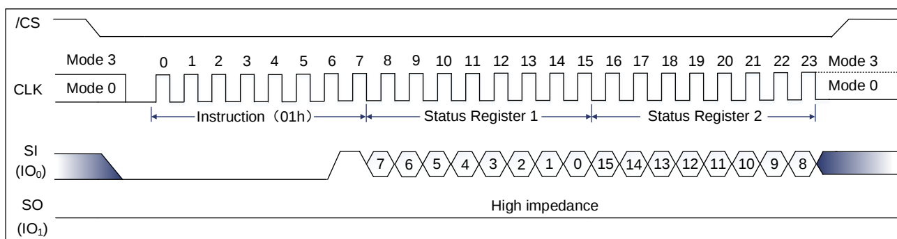
Figure 9-8 Write Status Register-1/2 Instruction (SPI Mode)
