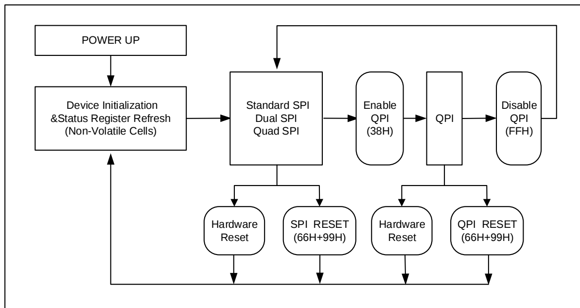
Figure 7-1 WX25QH32D Serial Flash Memory Operation Diagram
