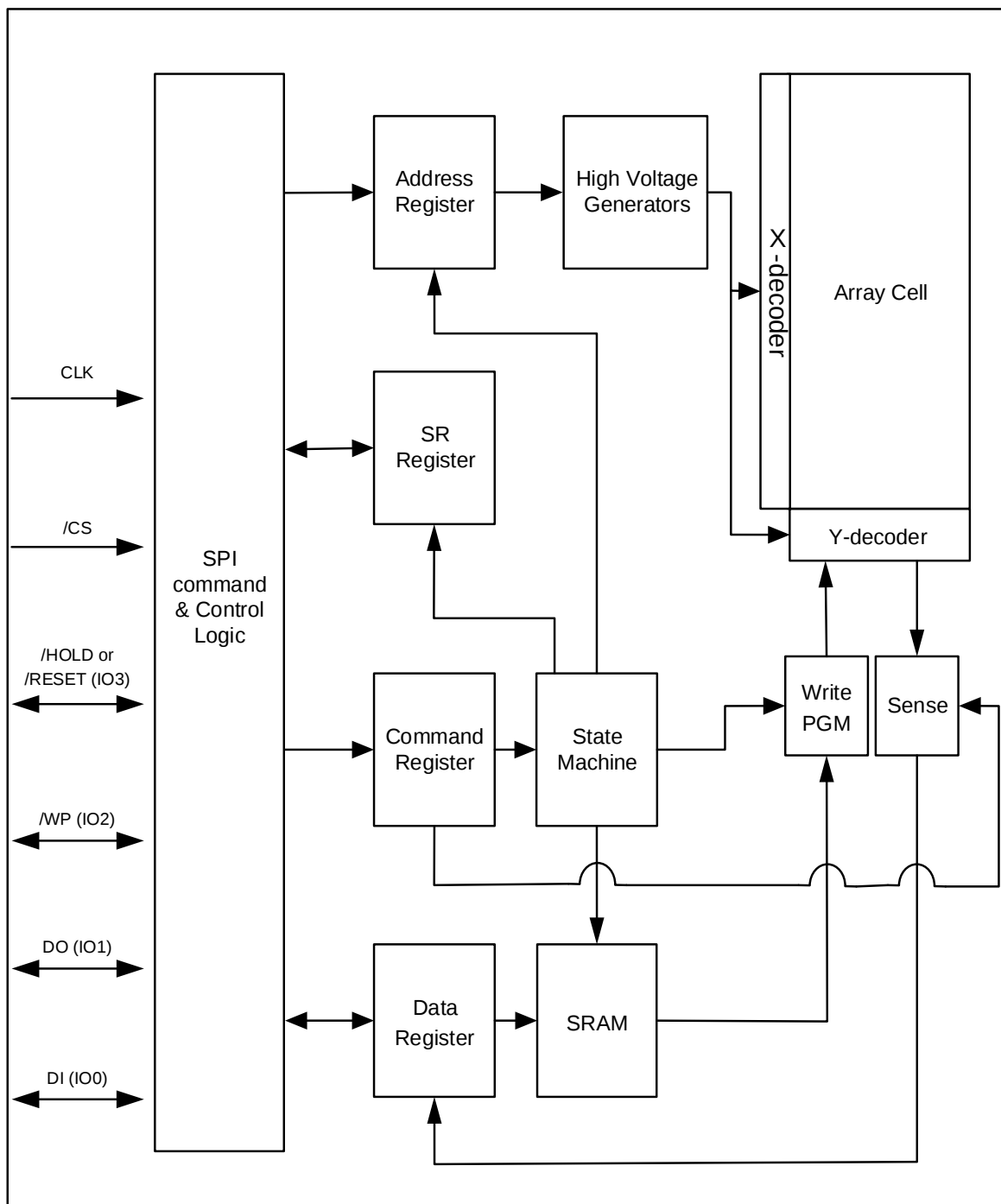
Figure 4-1 WX25QH32D Serial Flash Memory Block Diagram
