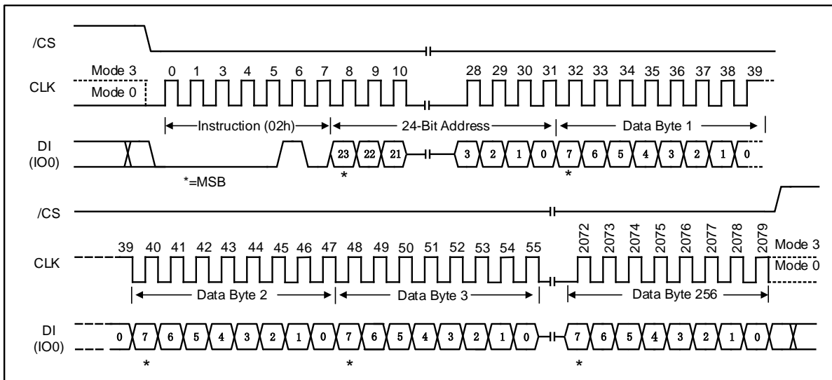
Figure 18a. Page Program Instruction (SPI Mode)
