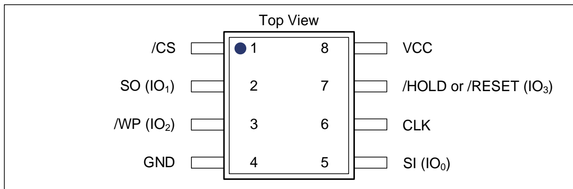
Figure 5-1 8-pin SOP 208-mil (Package Code H)
