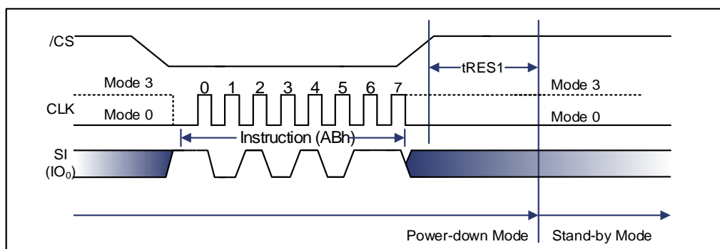
Figure 9-47 Release Power-down Instruction (QPI Mode)
