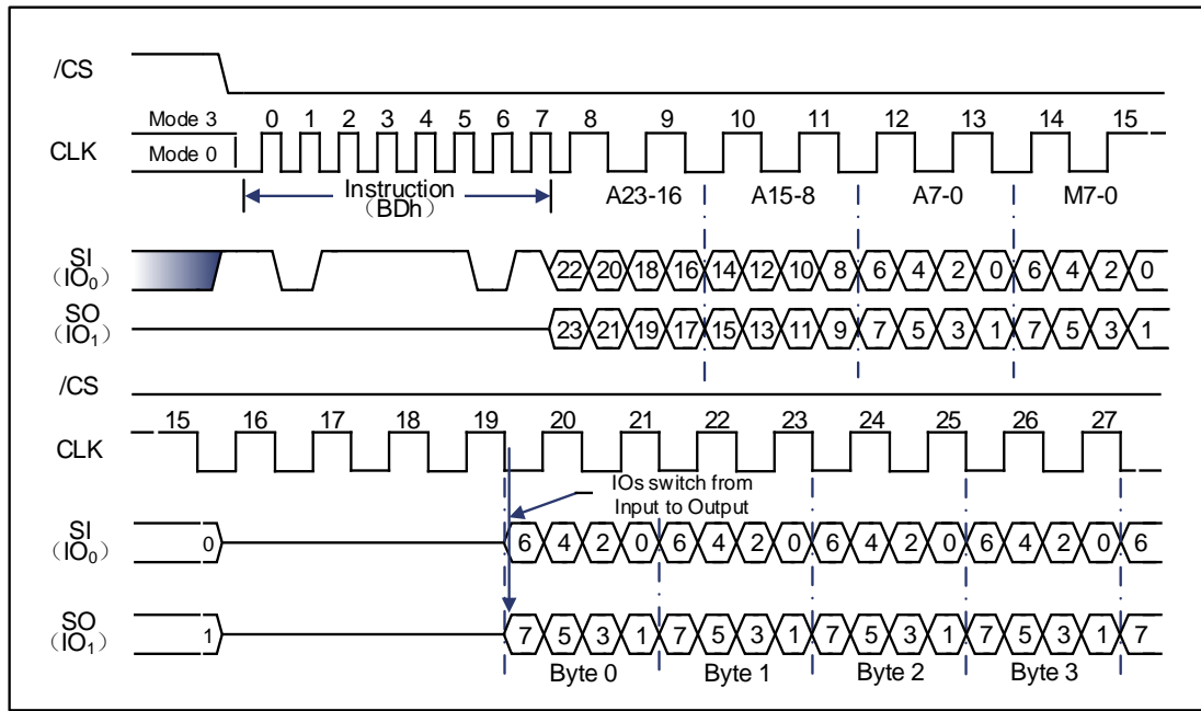
Figure 9-20 DTR Fast Read Dual I/O (Previous instruction set M5-4#10, SPI Mode only)
