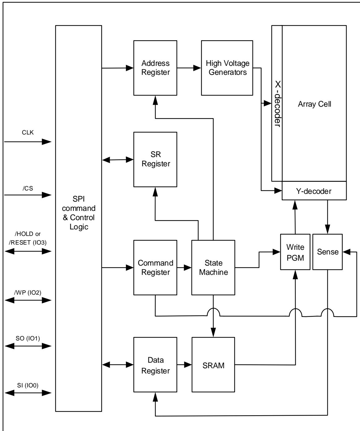
Figure 4-1 XM25QH32D Serial Flash Memory Block Diagram
