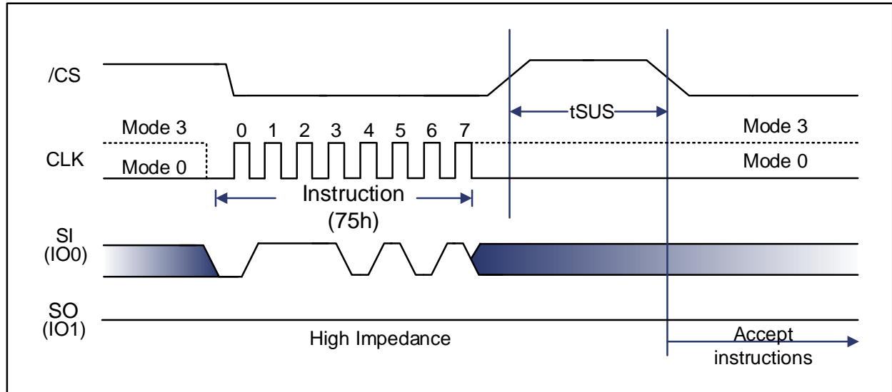
Figure 9-40 Erase/Program Suspend Instruction (SPI Mode)
