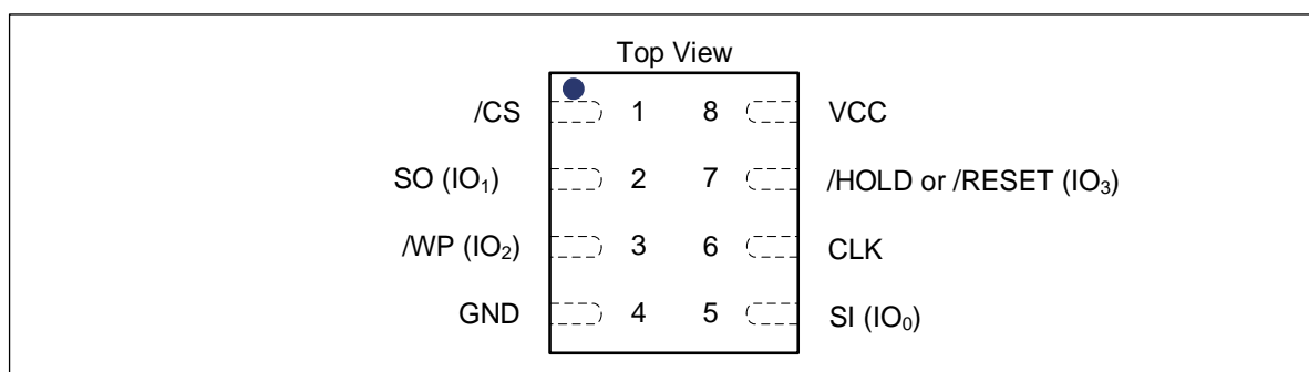
Figure 5-2 8-pad USON & WSON (Package Code U, U2 and W)
