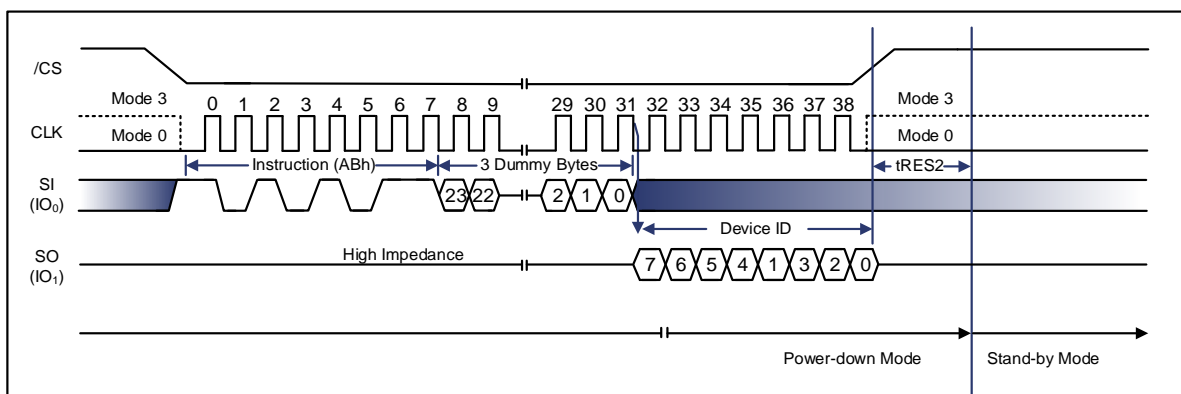
Figure 9-48 Release Power-down / Device ID Instruction (SPI Mode)
