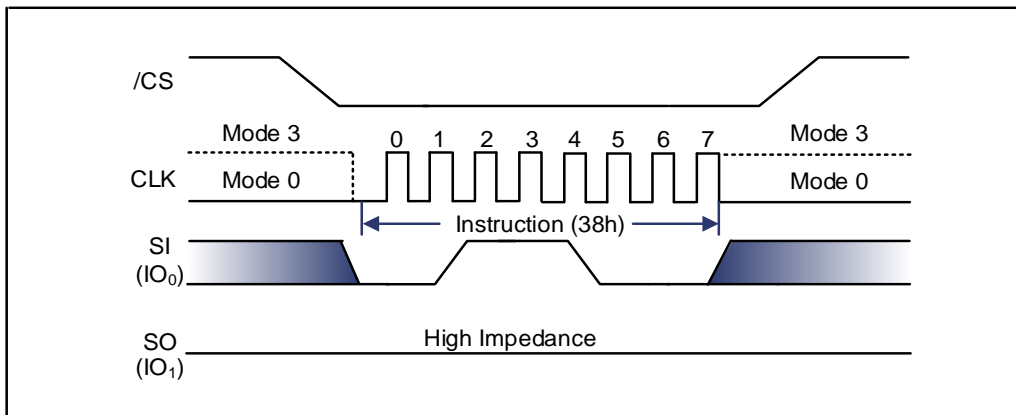
Figure 9-63 Enter QPI Instruction (SPI Mode only)
