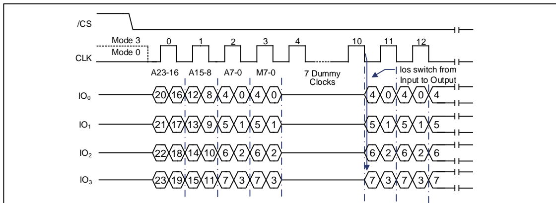
Figure 9-24 DTR Fast Read Quad I/O (Previous instruction set M5-4#10, SPI Mode)
