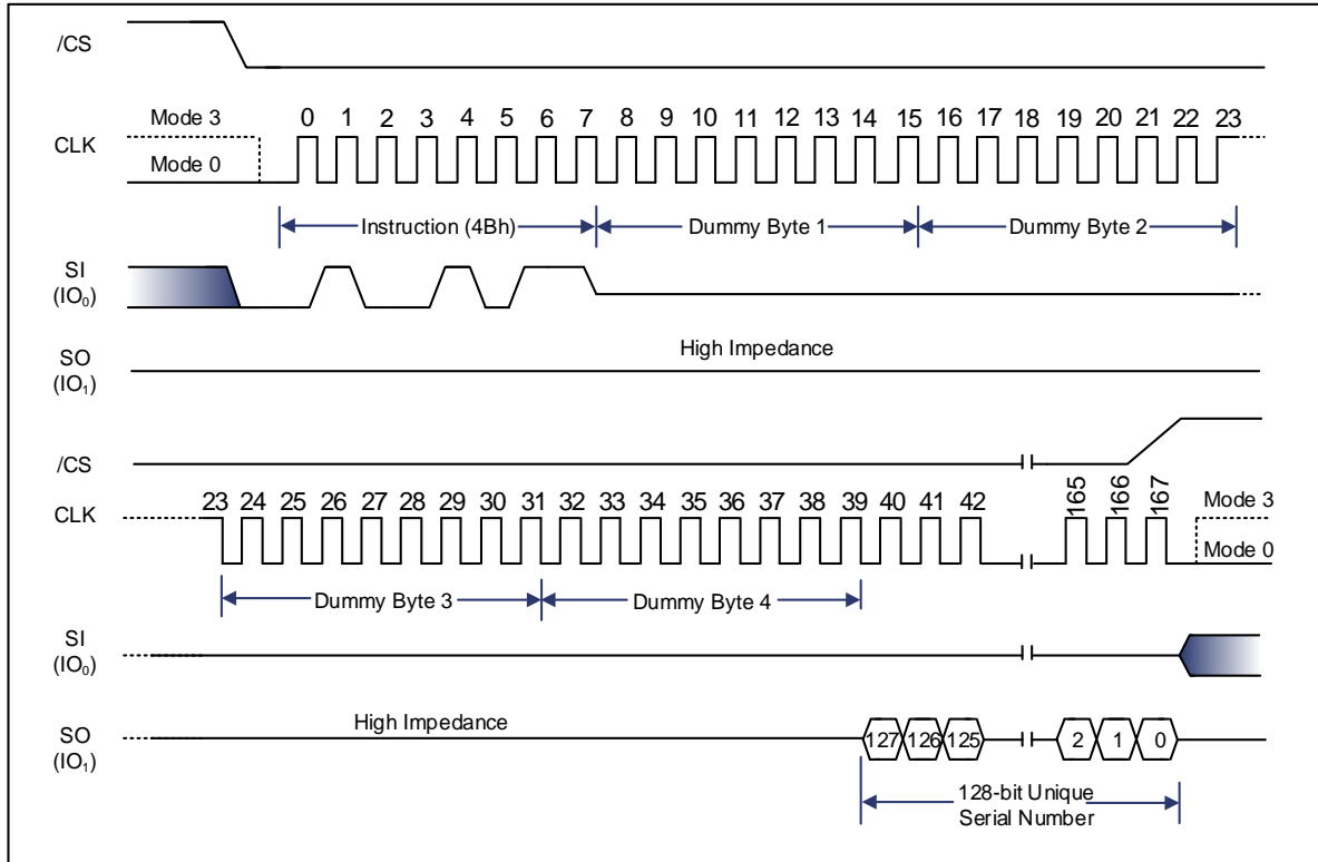
Figure 9-53 Read Unique ID Number Instruction (SPI Mode only)
