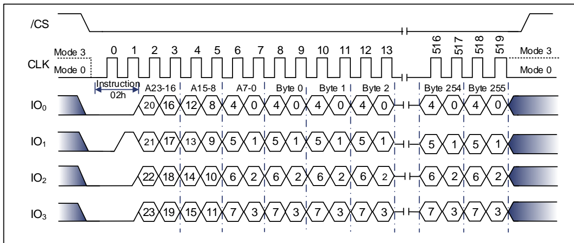
Figure 9-31 Page Program Instruction (QPI Mode)
