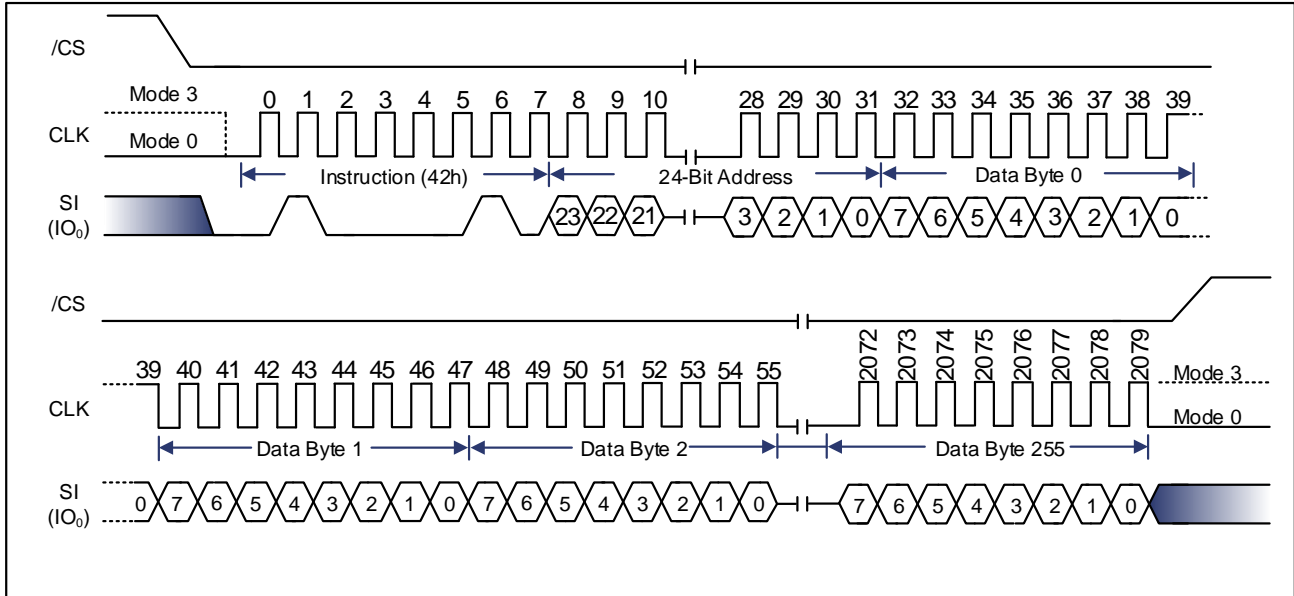
Figure 9-58 Program Security Registers Instruction (SPI Mode only)
