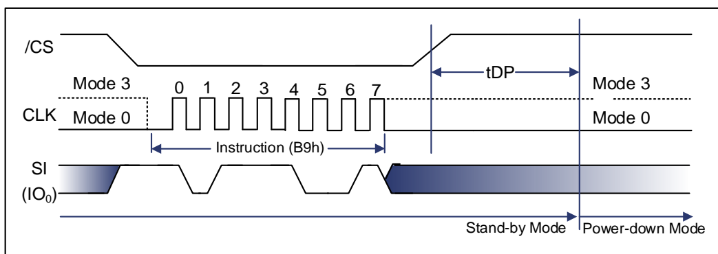
Figure 9-44 Deep Power-down Instruction (SPI Mode)
