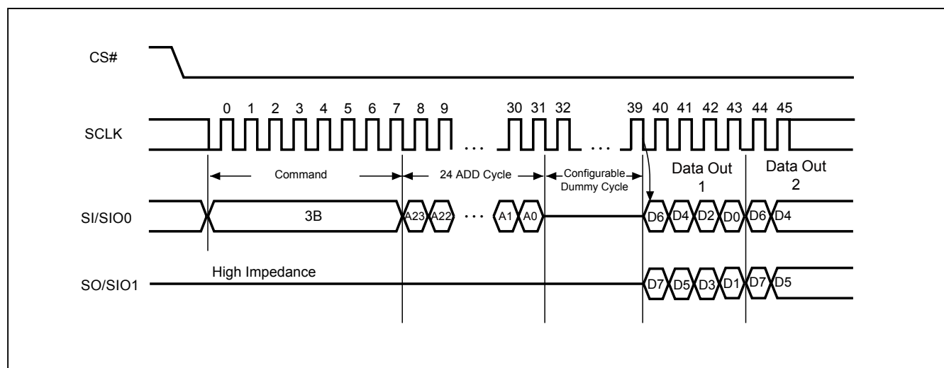
Figure 35. Dual Read Mode Sequence (SPI Mode only)
