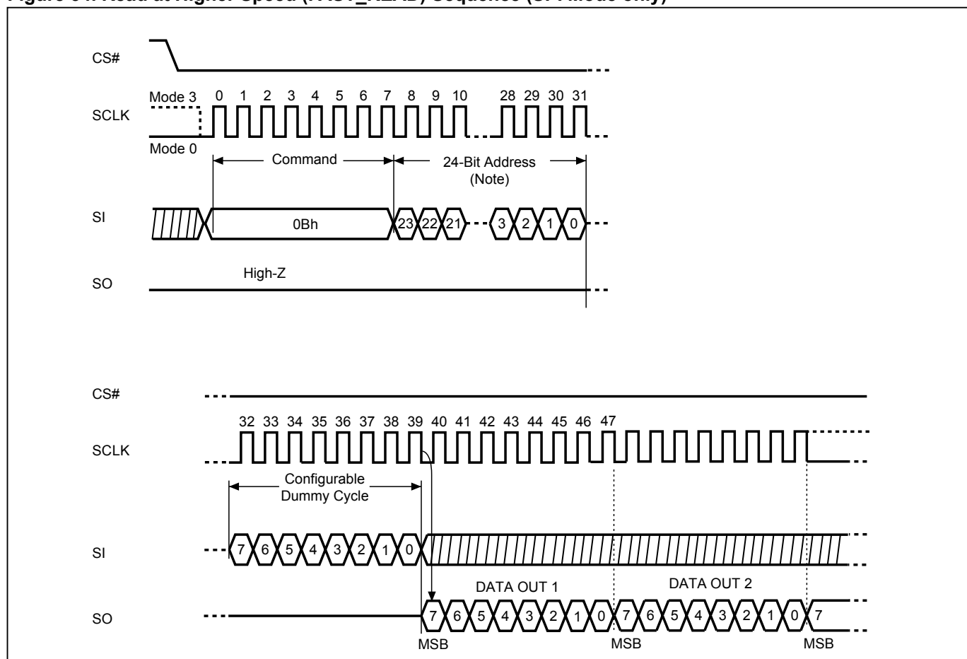
Figure 34. Read at Higher Speed (FAST_READ) Sequence (SPI Mode only)
