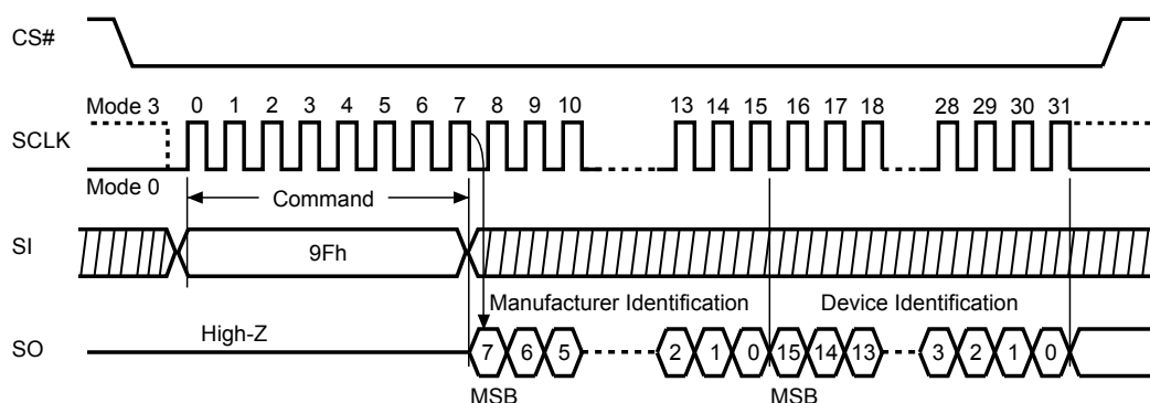
Figure 17. Read Identification (RDID) Sequence (SPI mode only)
